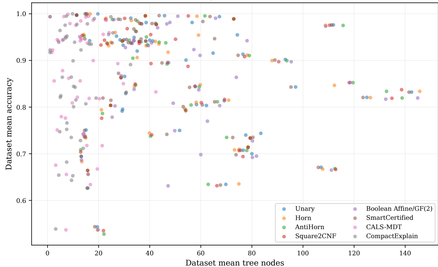
Accuracy versus tree nodes
