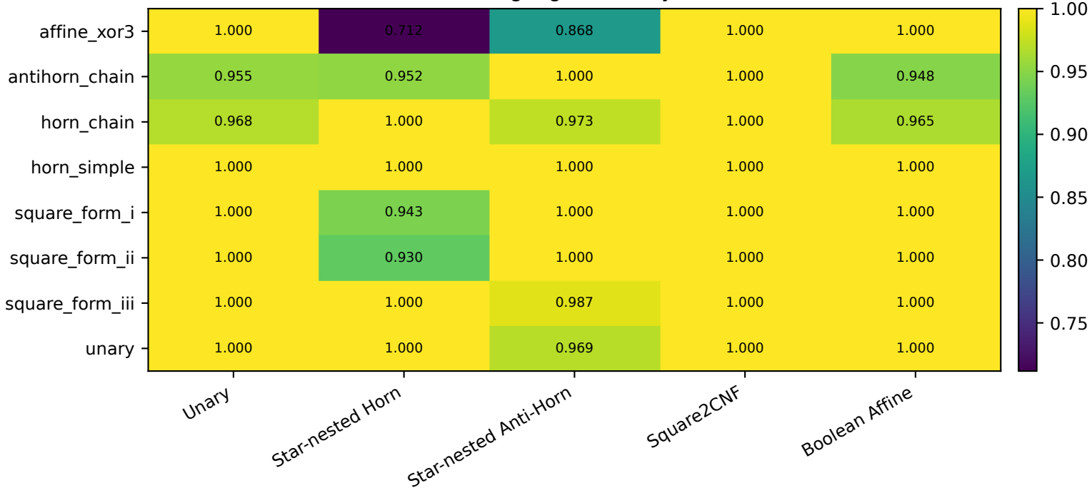
Controlled exact-language accuracy (0% label noise)
