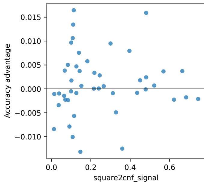
Square2CNF: \rho=0.14
