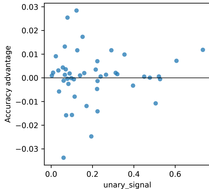
Square2CNF: \rho=0.14
