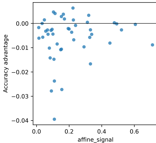
Boolean Affine: \rho=0.11
