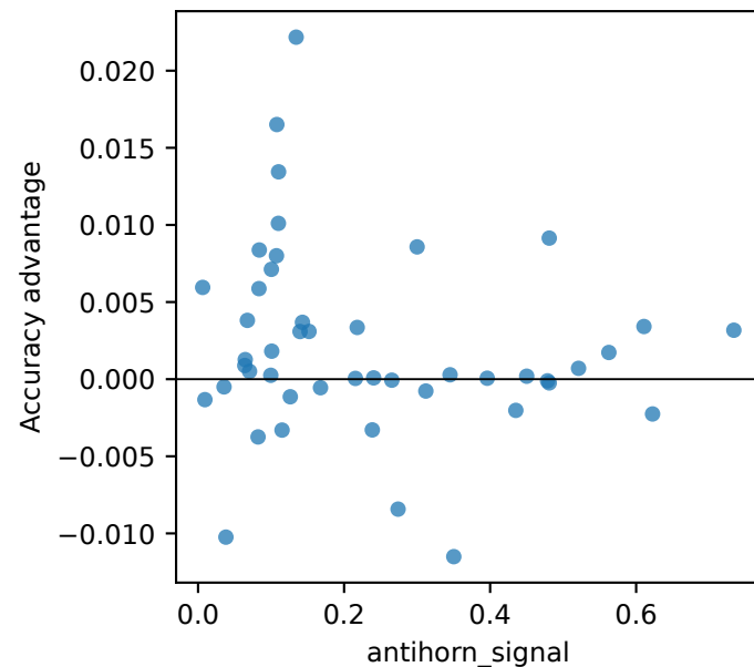
Star-nested Anti-Horn: \rho=-0.14
