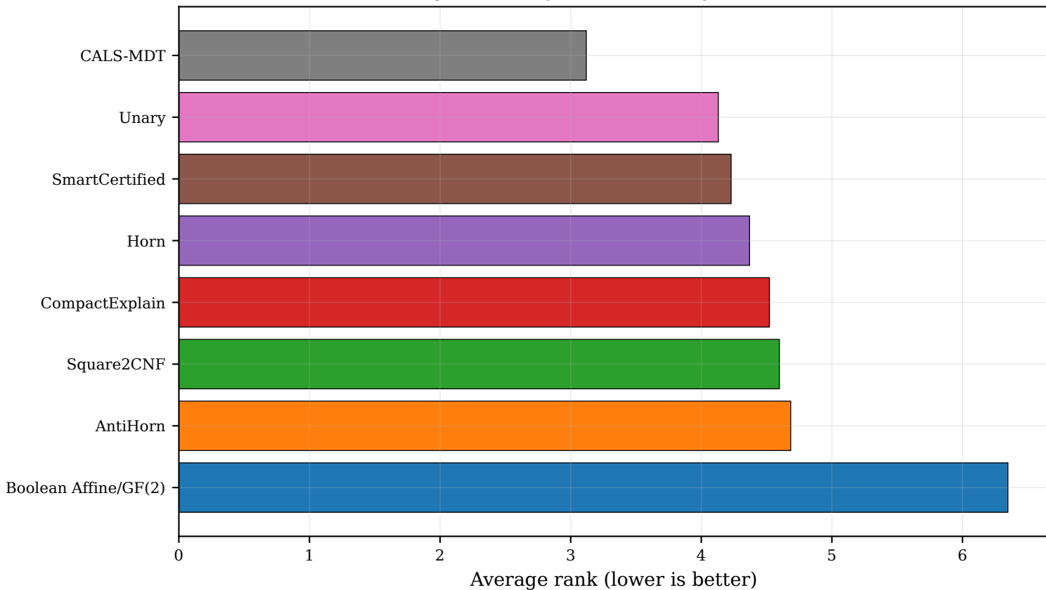
Average accuracy rank (Nemenyi CD = 1.548)
