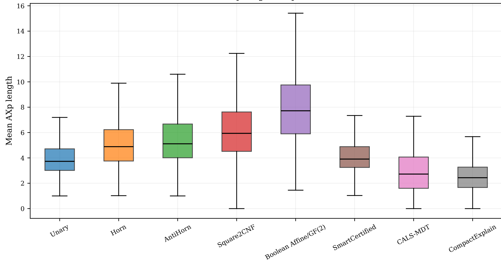
AXp-length boxplot
