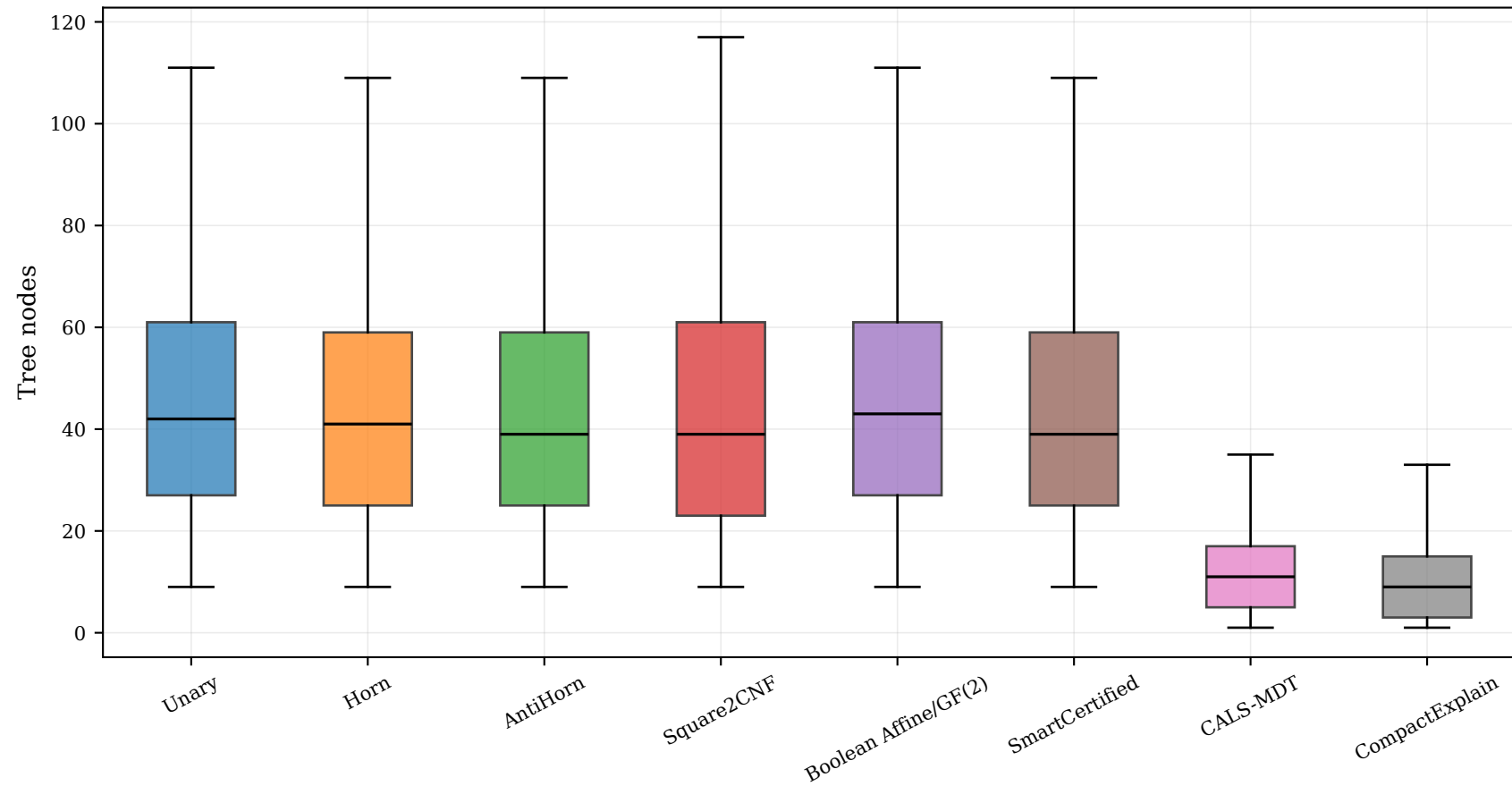
Tree-node boxplot
