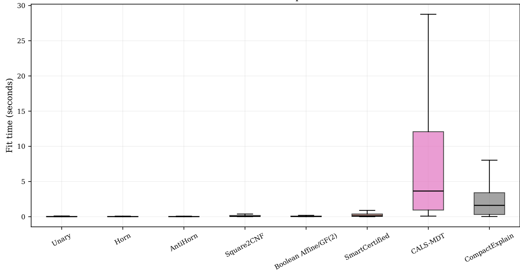
Runtime boxplot
