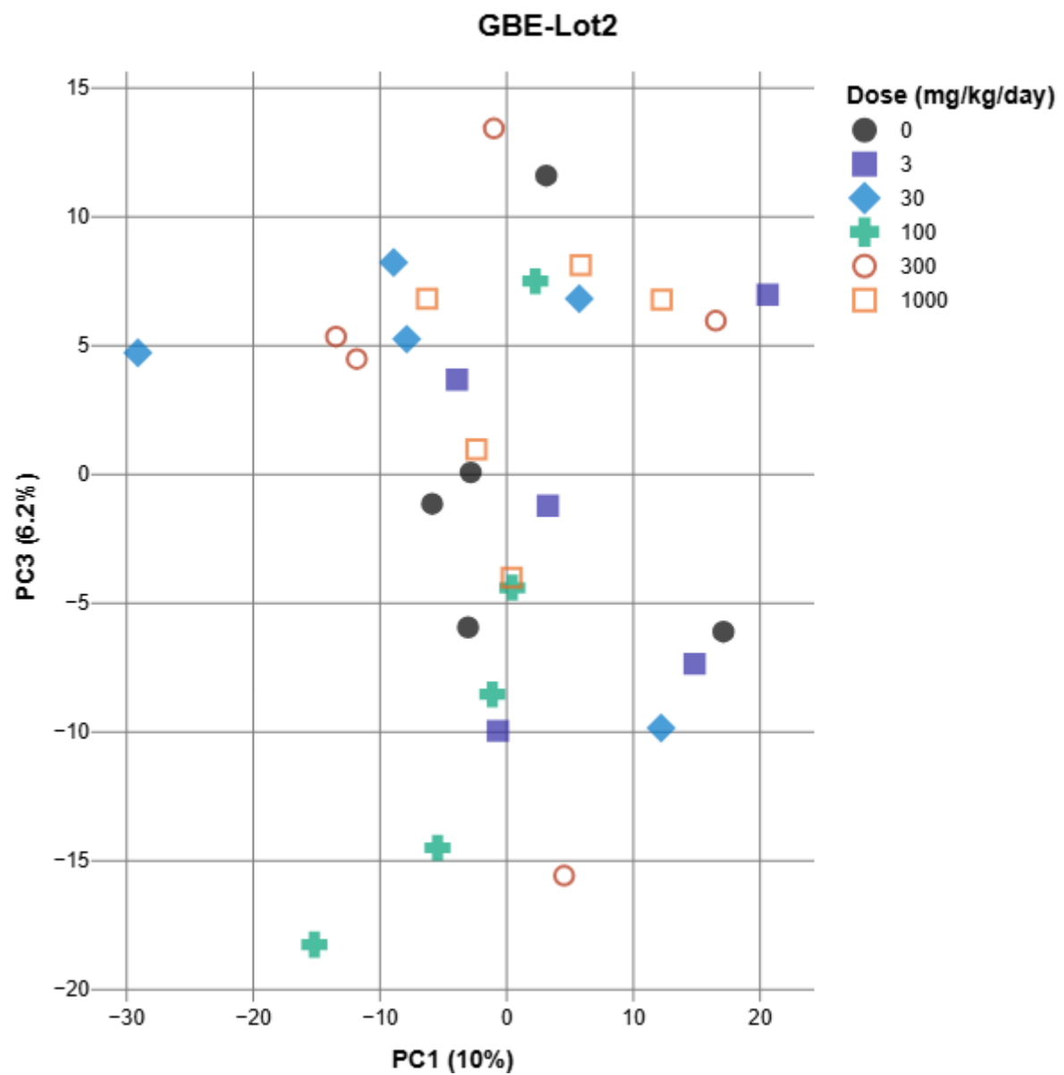
Two-Dimensional Plot of PCA 1 Component vs. PCA 3 Component
