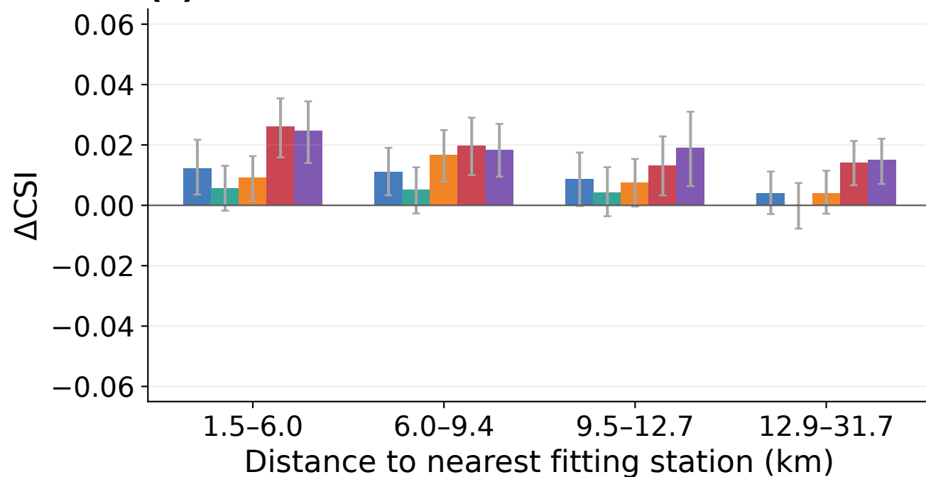
(c) RN60 \geq 10 mm
