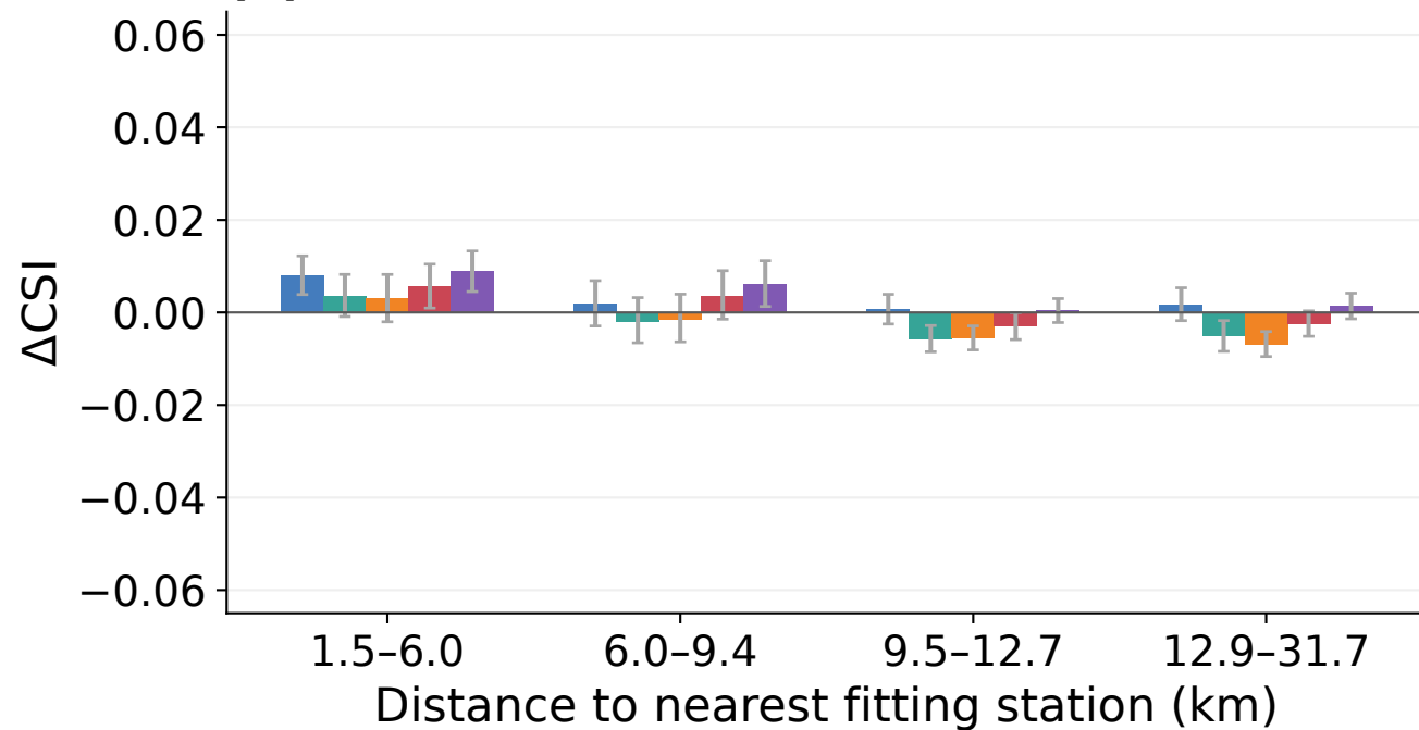
(a) RN60 \geq 1 mm
