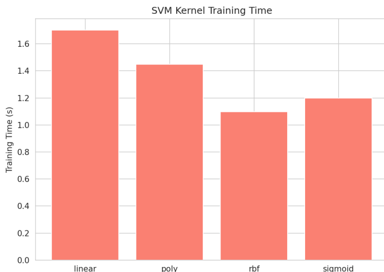
Figure 8: SVM training time by kernel.
