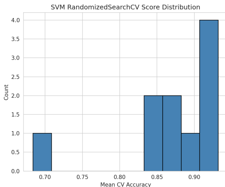
Figure 10: Distribution of mean CV accuracy across the 10 RandomizedSearchCV samples for SVM.
