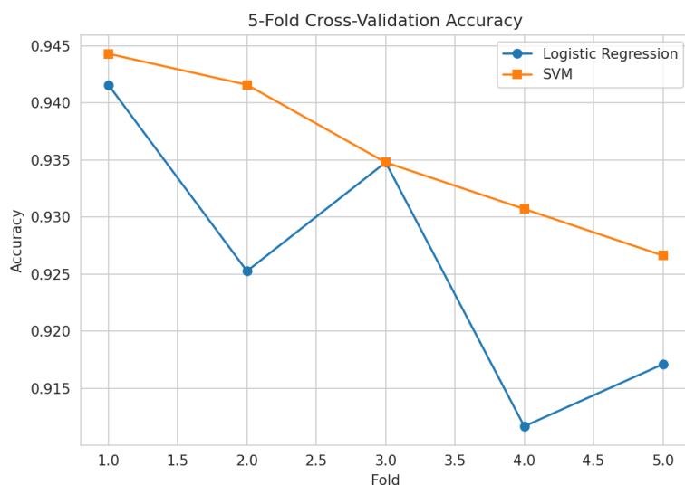
Figure 11: Per-fold cross-validation accuracy, Logistic Regression vs. SVM.
