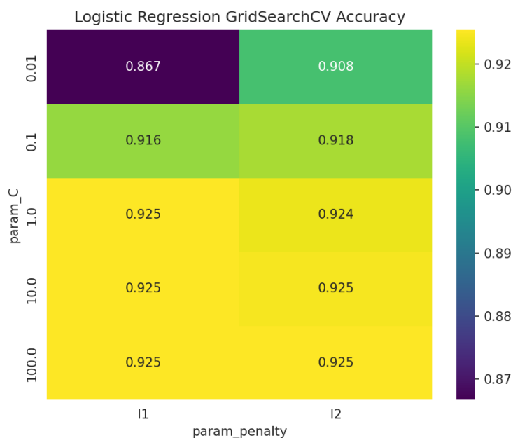
Figure 9: GridSearchCV mean CV accuracy for Logistic Regression, by C and penalty.
