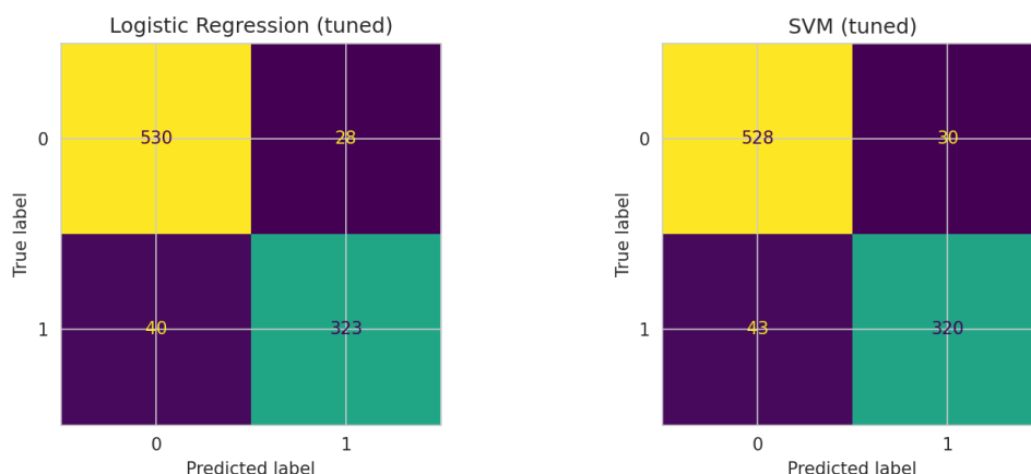
Figure 5: Confusion matrices for the tuned Logistic Regression and tuned SVM on the test set.
