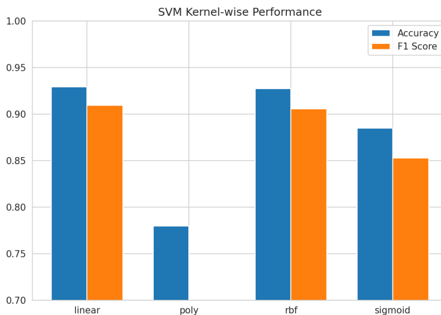
Figure 7: Accuracy and F1-score across all four SVM kernels (default hyperparameters).
