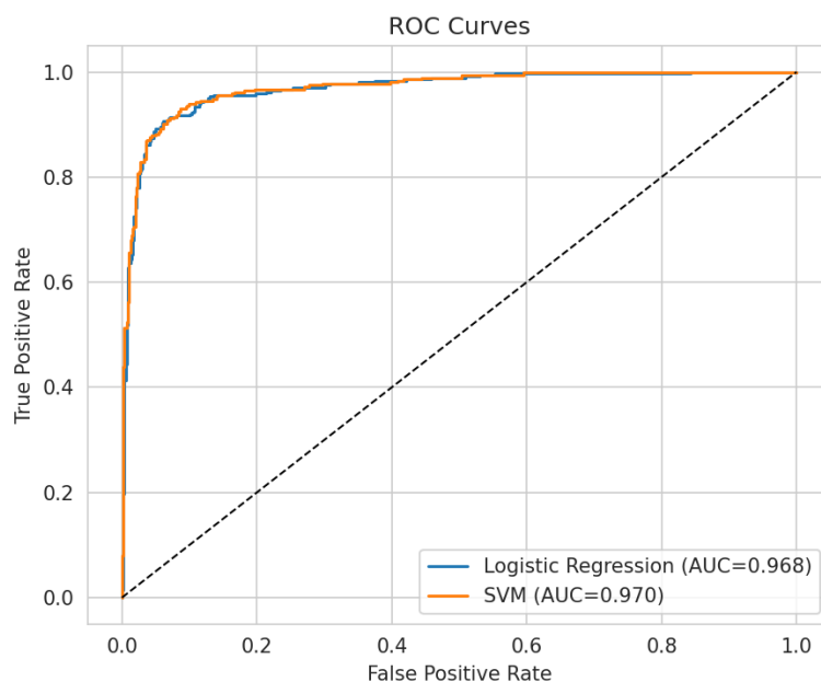
Figure 6: ROC curves for tuned Logistic Regression and tuned SVM.
