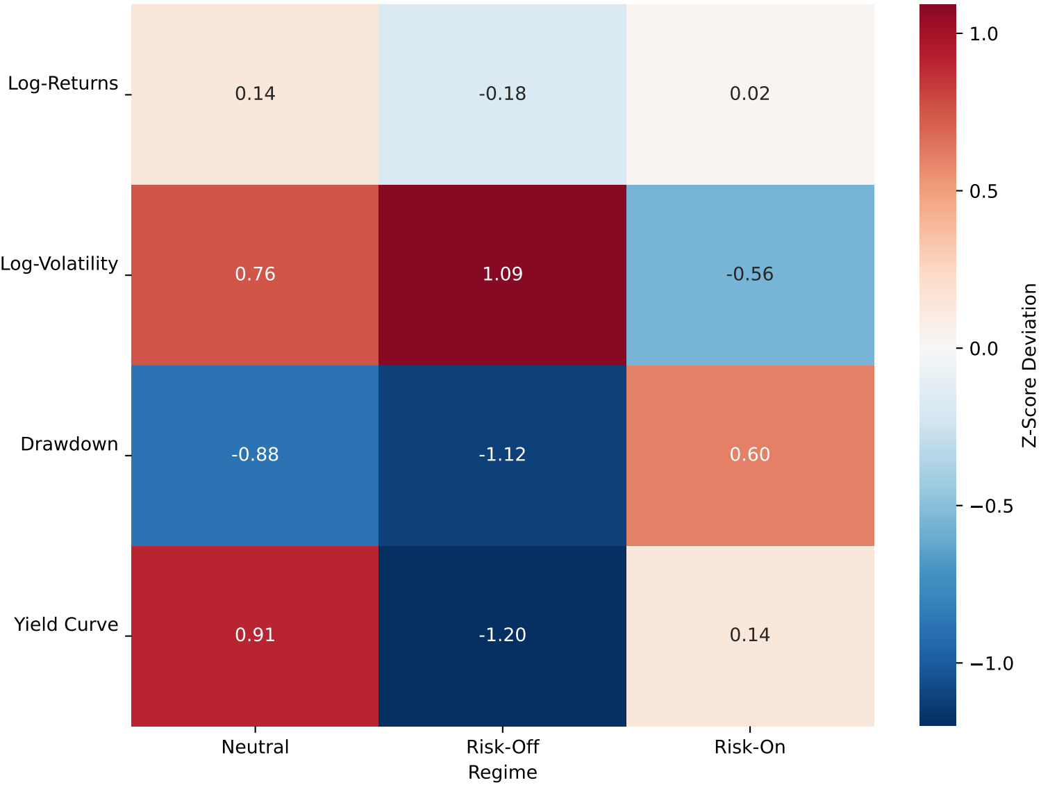
2. Regime Characteristics (Feature Means)
