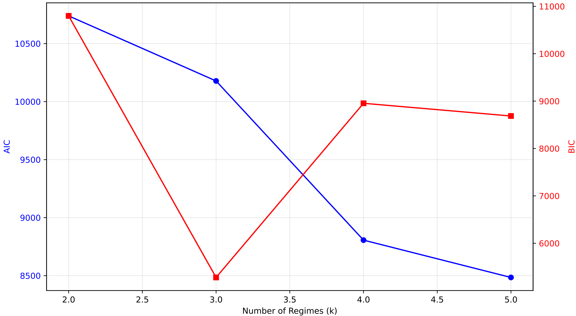
Model Selection: AIC vs BIC
