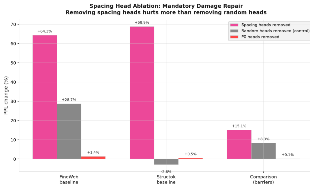
Figure 10: Figure 9: Ablation comparison across three models.
