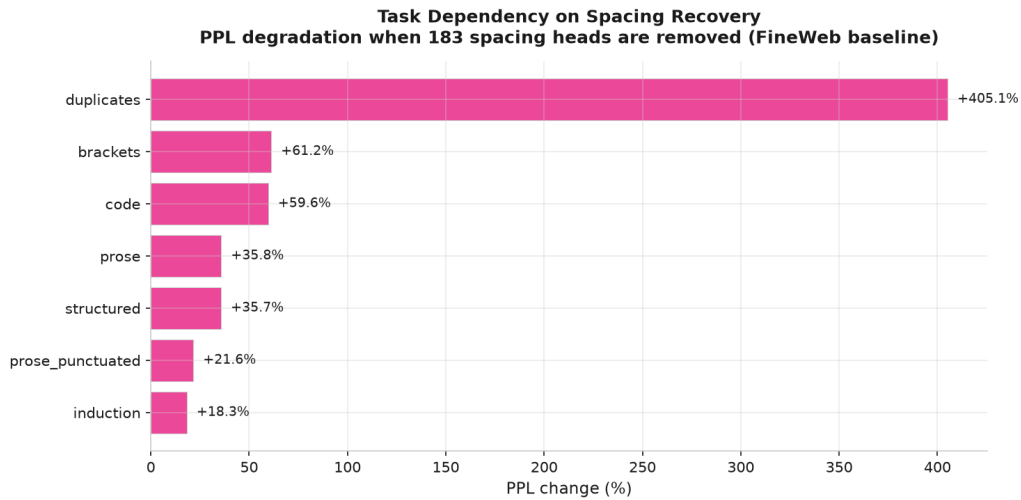
Figure 9: Figure 11: Per-text degradation when spacing heads are removed (FineWeb baseline). Duplicate detection depends most on whitespace boundary recovery (+405%), followed by code and brackets (~60%), then prose (~35%).
