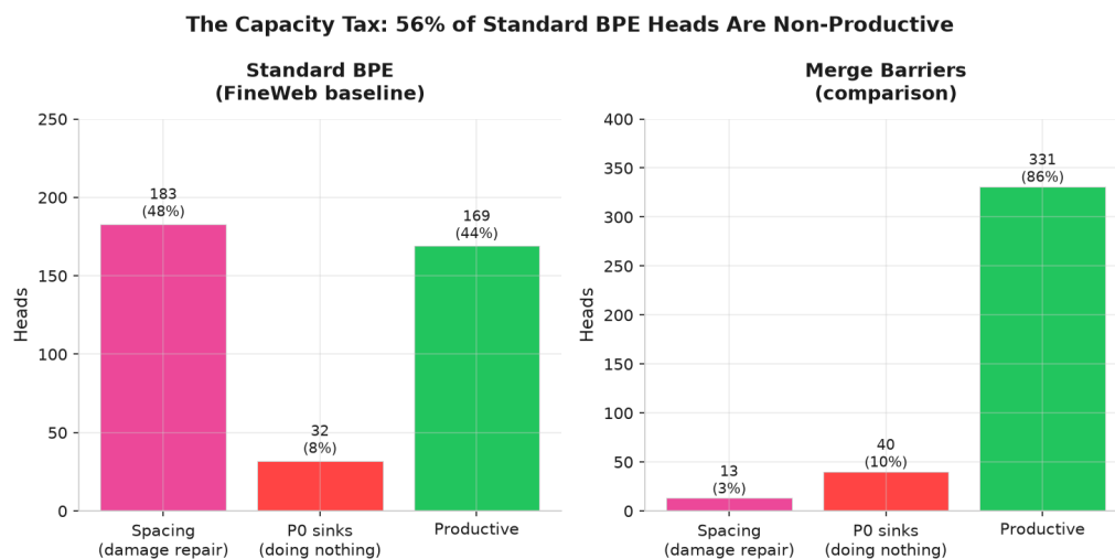
Figure 11: Figure 12: The capacity tax. Standard BPE baseline (left): 183 heads on mandatory spacing recovery, 32 on P0 collapse, 169 productive. Merge-barrier comparison (right): 13 spacing, 40 P0, 331 productive. Merge barriers convert the spacing tax into available capacity.
