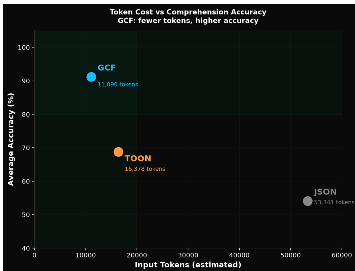
Figure 7: Token Cost vs Comprehension Accuracy
