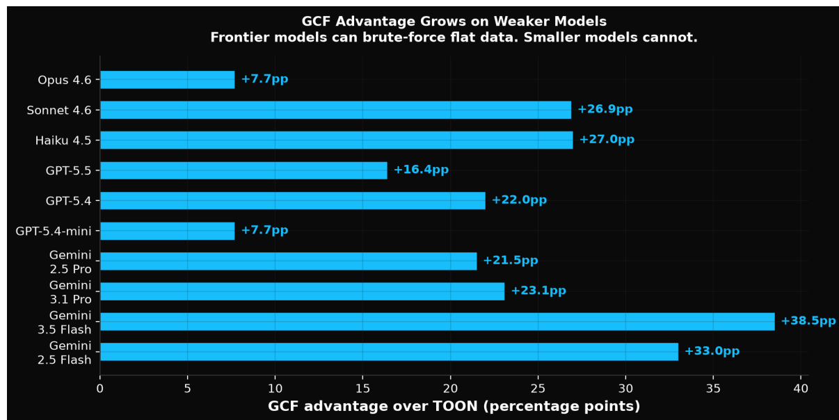
Figure 12: GCF Advantage Grows on Weaker Models
