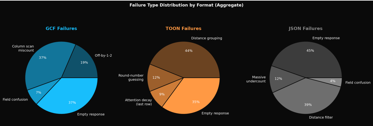
Figure 10: Failure Type Distribution
