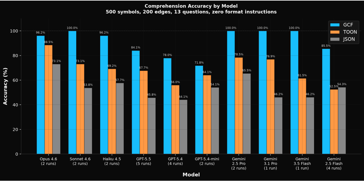
Figure 6: Comprehension Accuracy by Model
