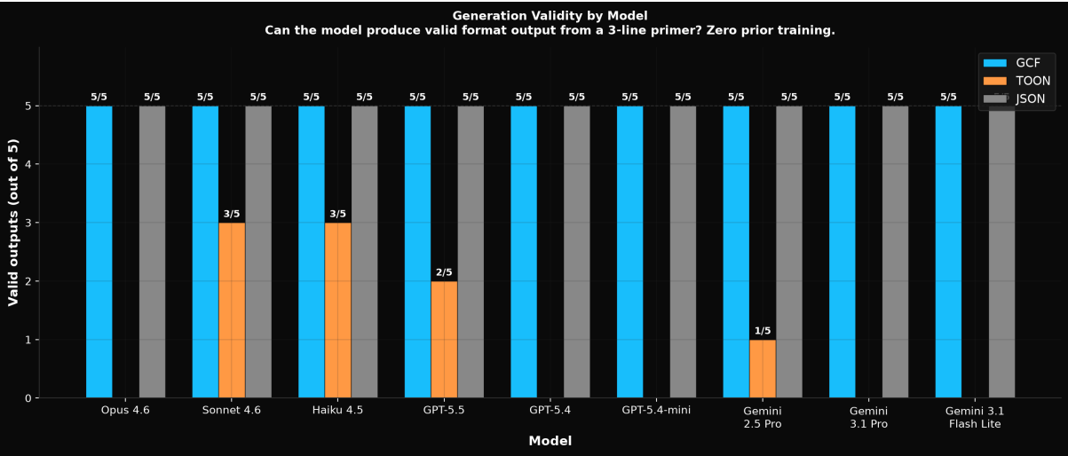
Figure 13: Generation Validity by Model
