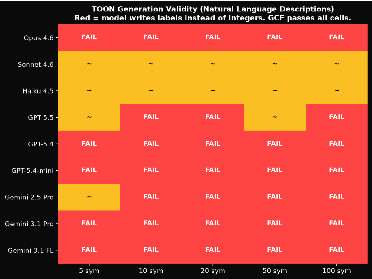
Figure 15: TOON Generation Heatmap
