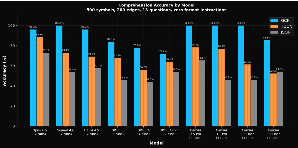
Figure 7: Comprehension Accuracy by Model
