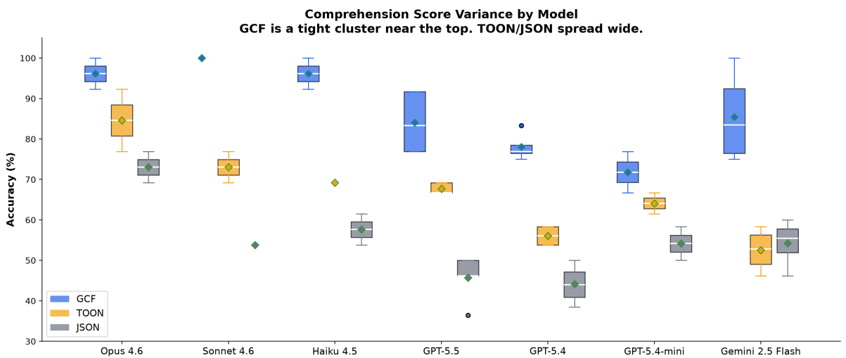
Figure 11: Comprehension Score Variance
