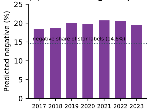
(b) Zero-shot negative predictions
