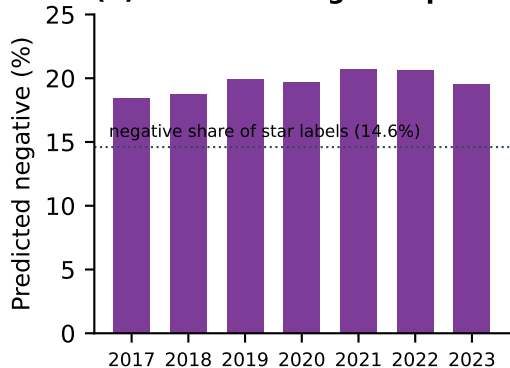
(b) Zero-shot negative predictions
