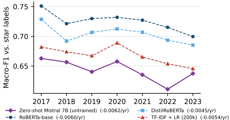
(a) Same 2,000 items per year
