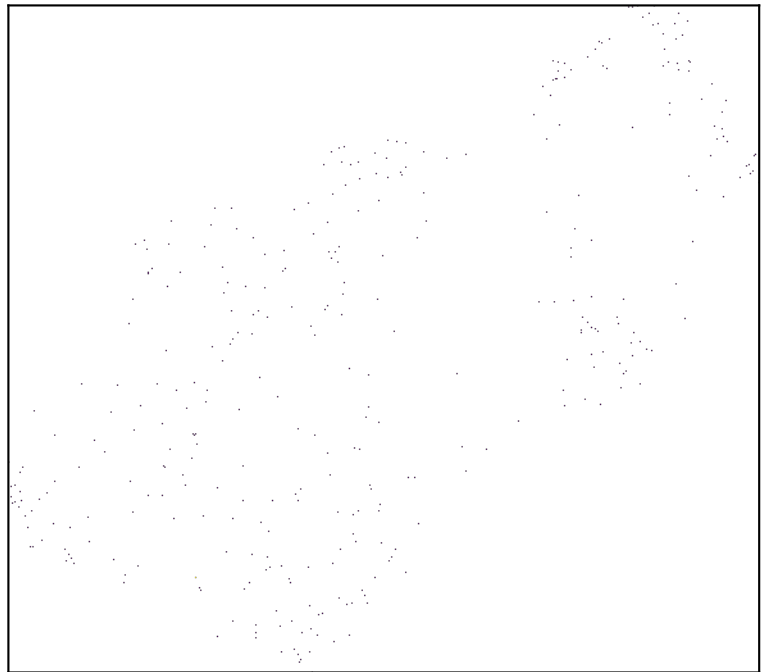
n_neighbors=200
