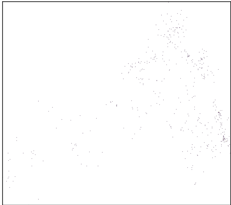
n_neighbors=60
