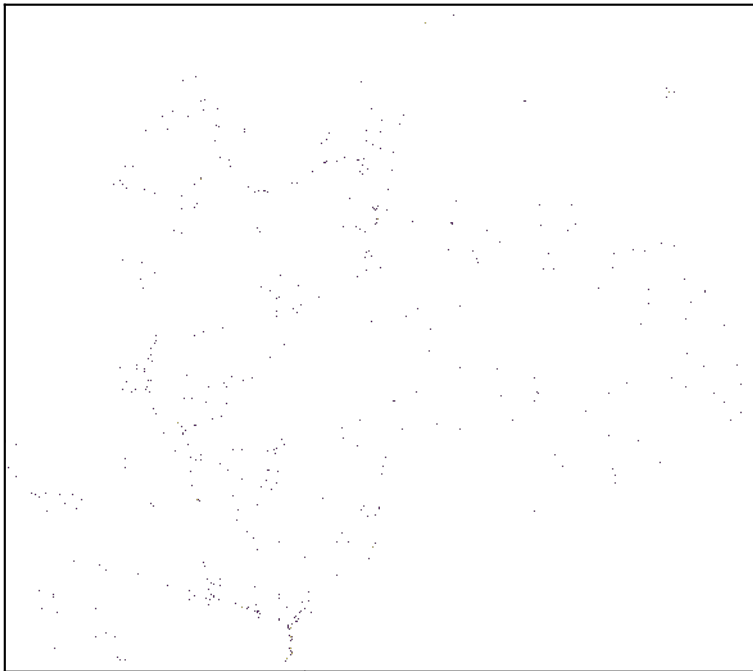
n_neighbors=6
