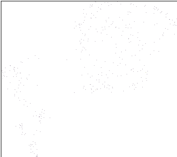
n_neighbors=90
