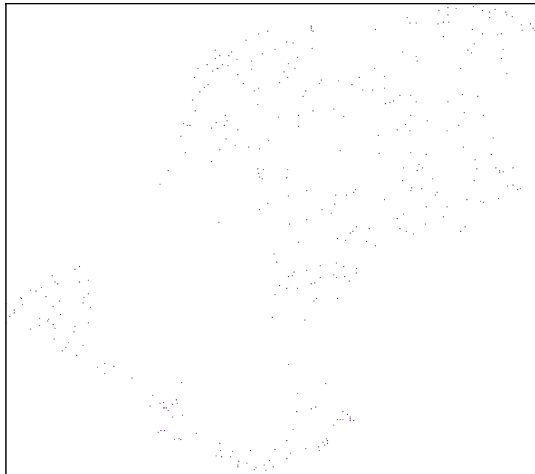
n_neighbors=60
