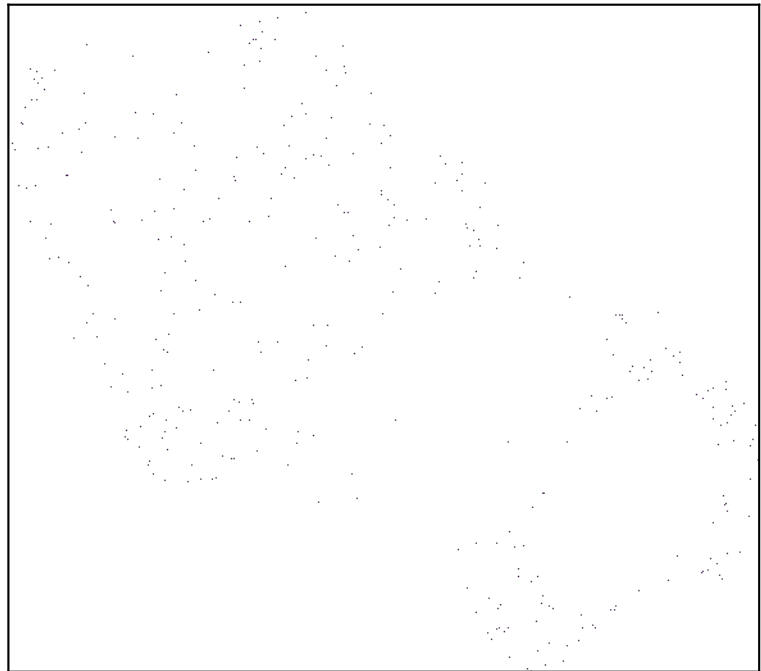
n_neighbors=100
