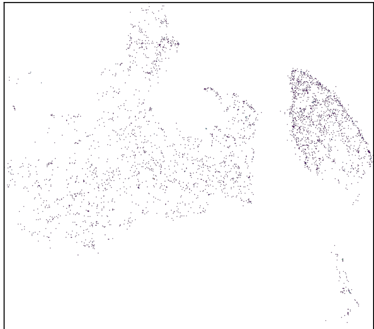
n_neighbors=60
