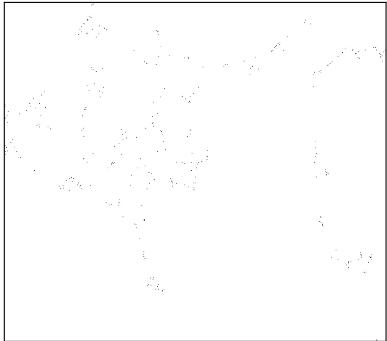
n_neighbors=7
