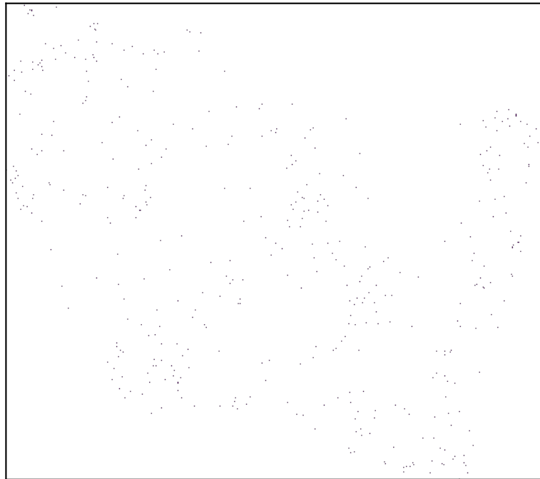
n_neighbors=100
