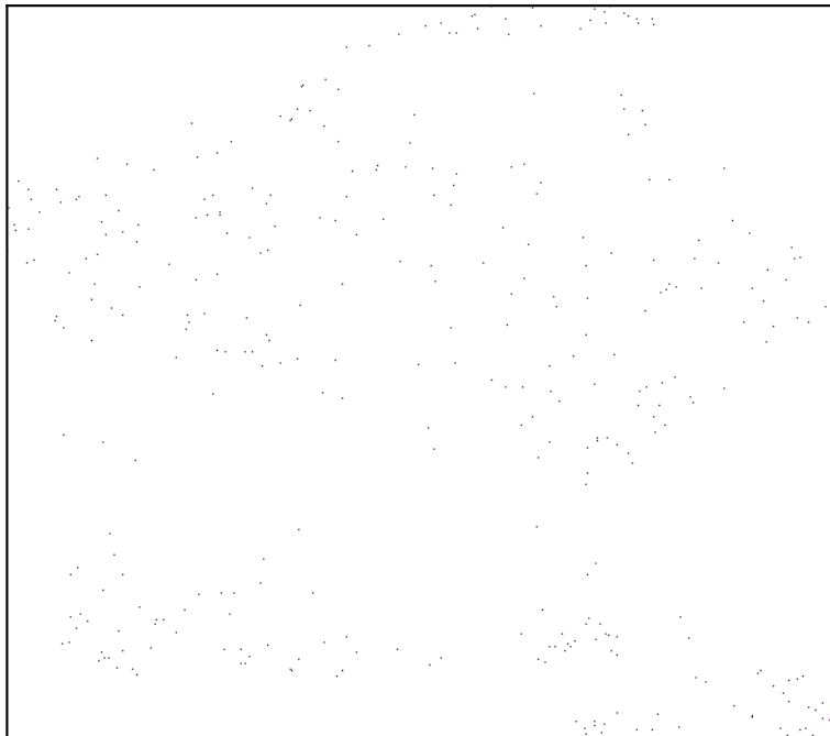
n_neighbors=200
