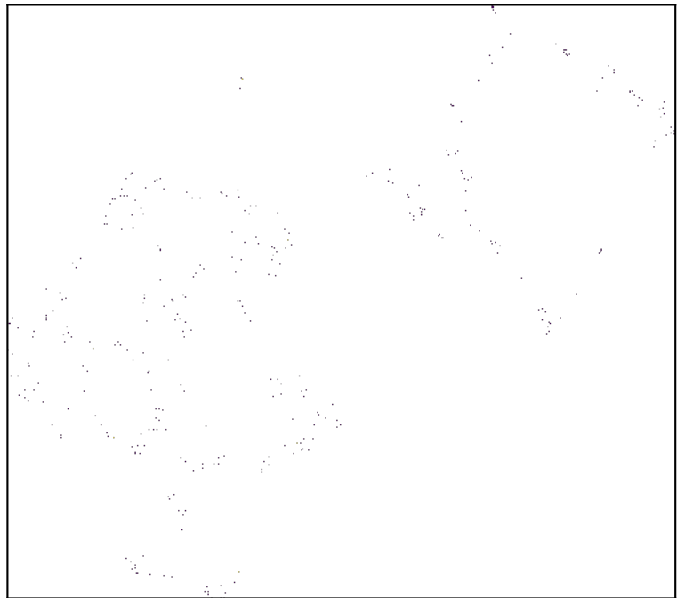
n_neighbors=9
