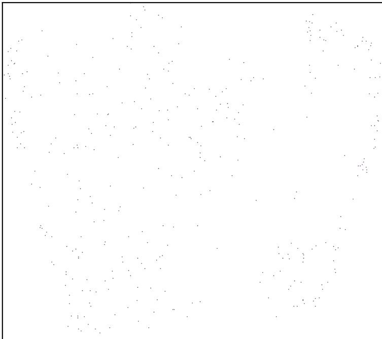
n_neighbors=150
