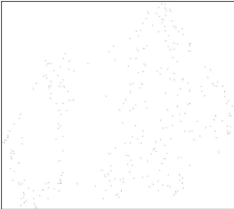
n_neighbors=90
