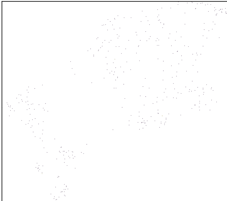
n_neighbors=100
