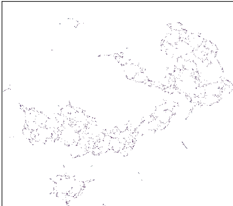
n_neighbors=7
