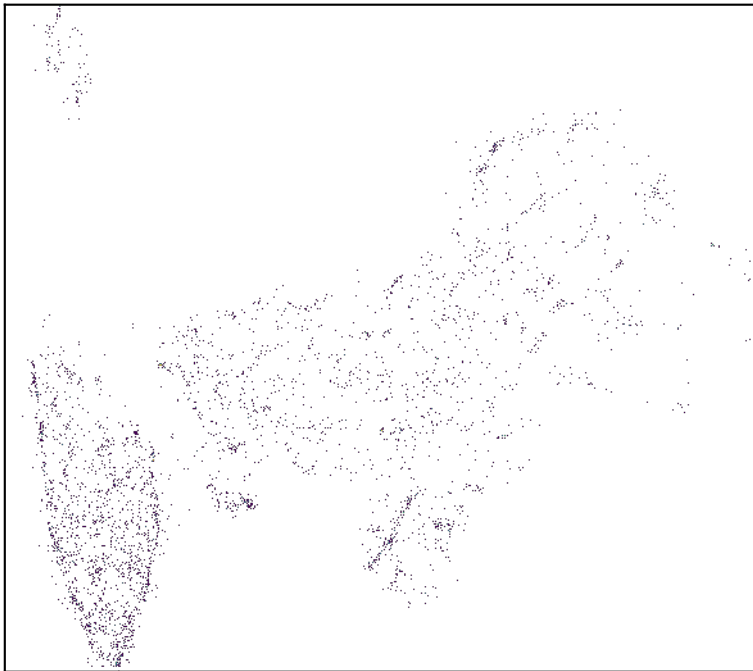
n_neighbors=350
