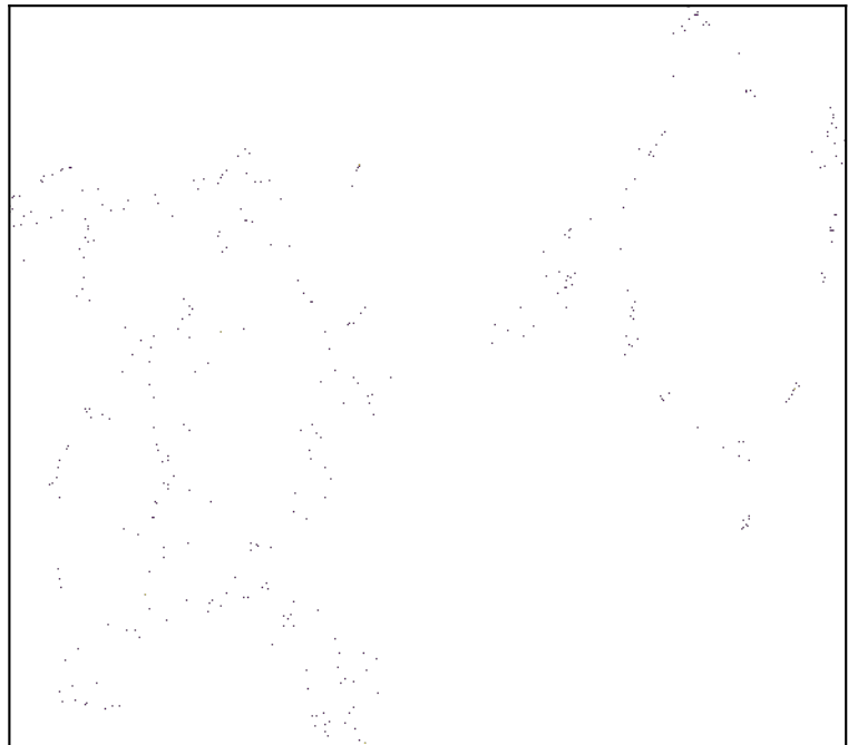
n_neighbors=9
