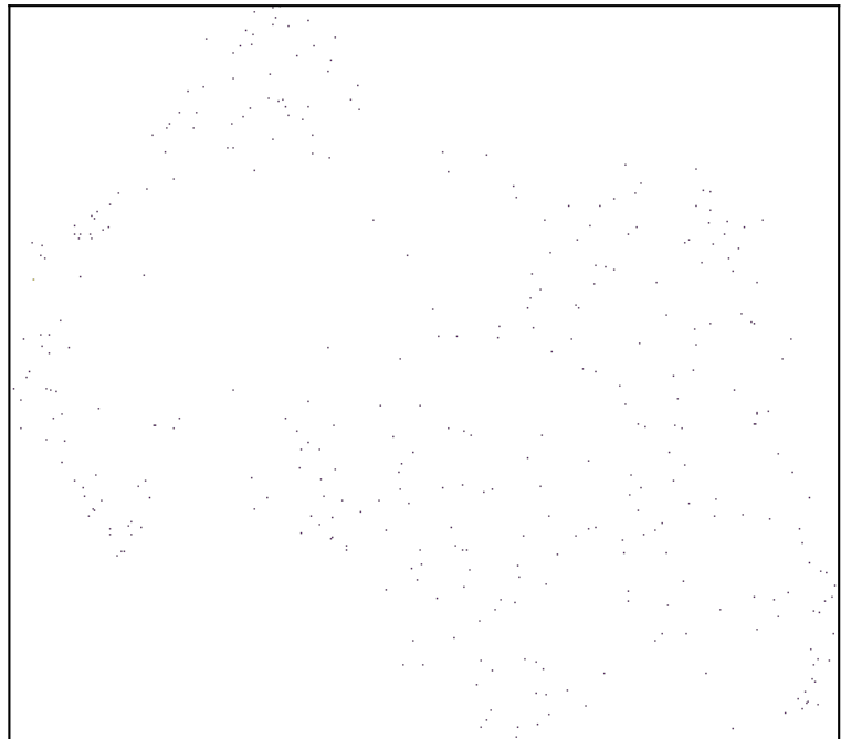
n_neighbors=200
