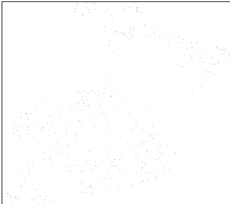
n_neighbors=200
