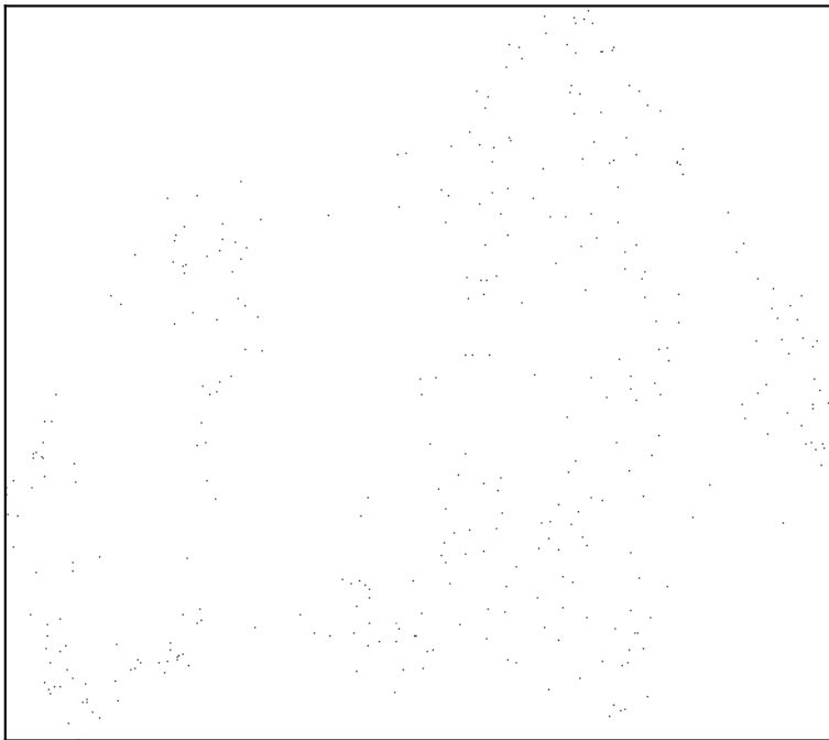
n_neighbors=150
