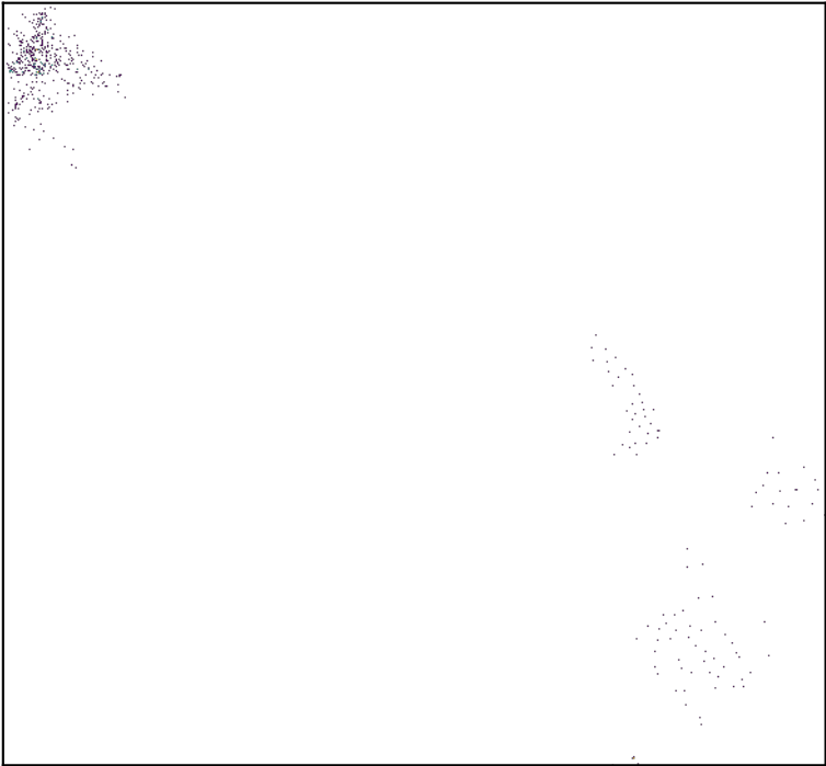
n_neighbors=250
