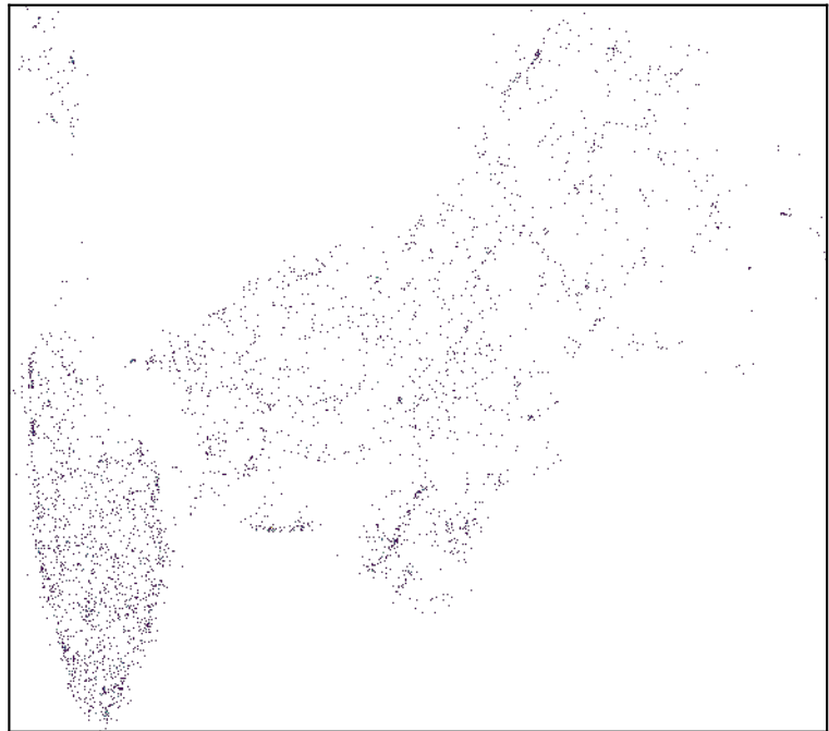
n_neighbors=400
