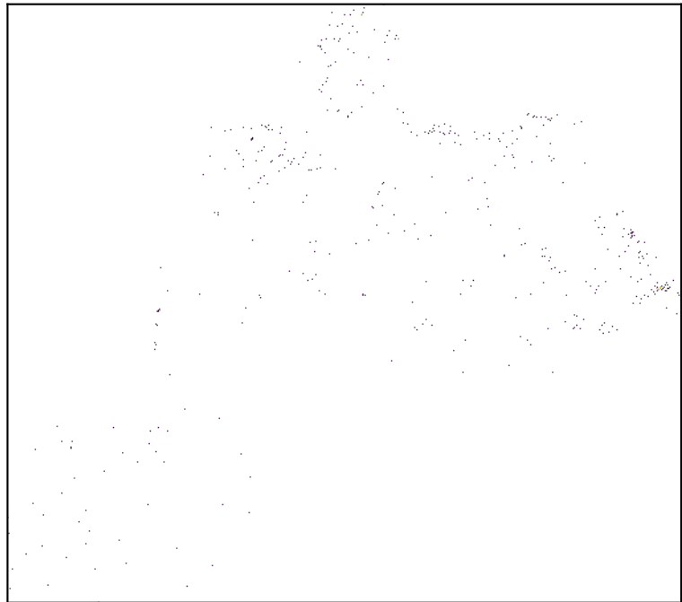
n_neighbors=40
