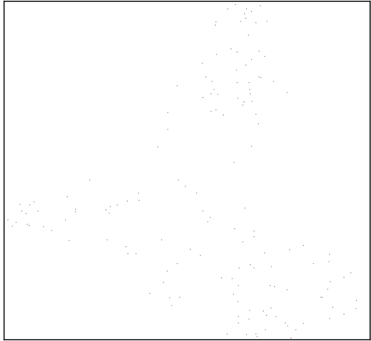
n_neighbors=80
