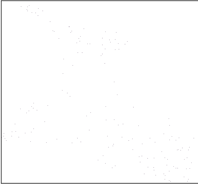
n_neighbors=70
