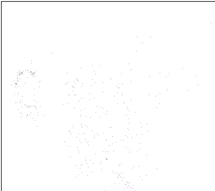
n_neighbors=50
