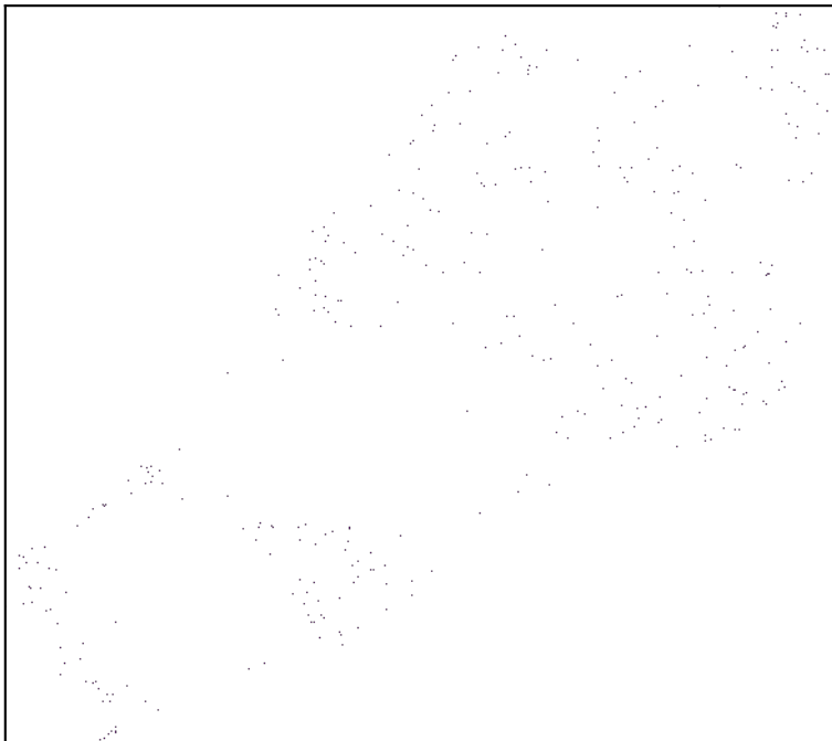
n_neighbors=50
