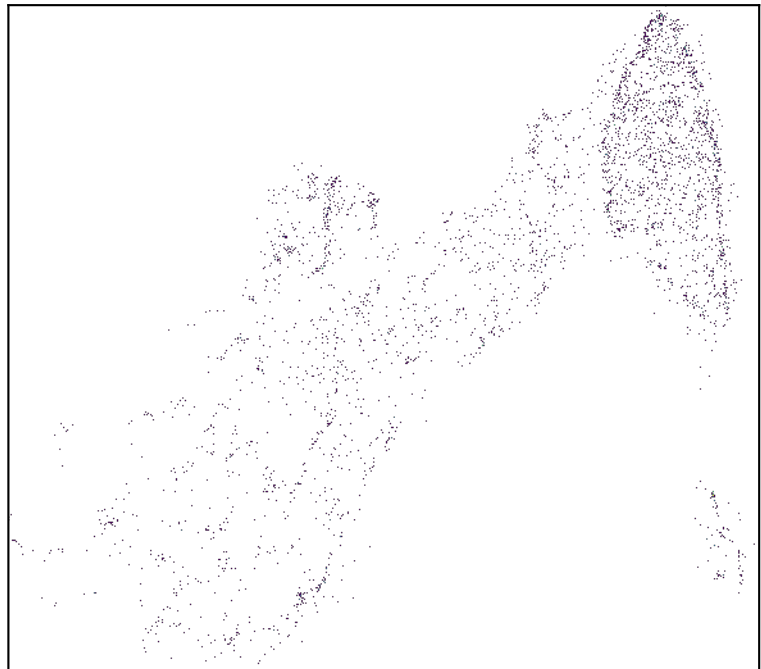
n_neighbors=500
