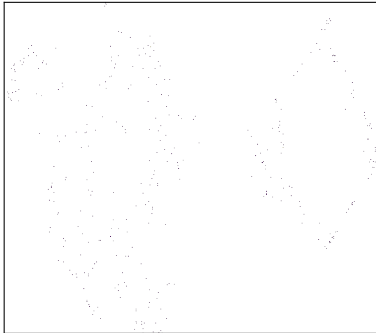
n_neighbors=40
