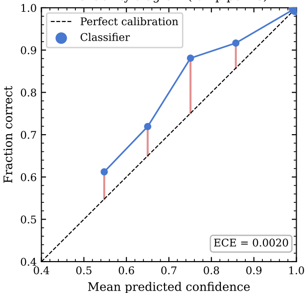
Reliability diagram (full pipeline)
