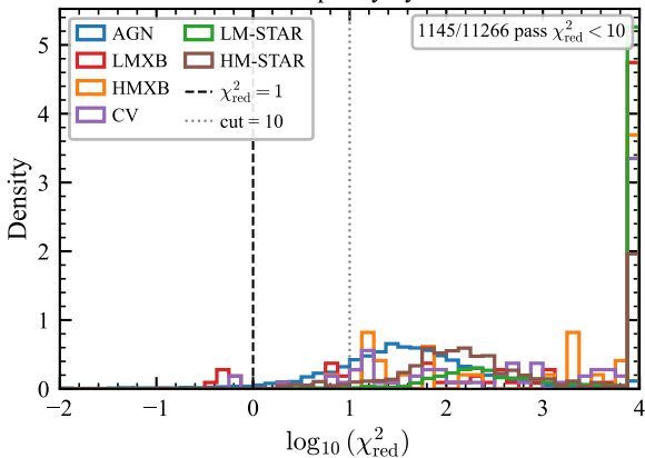
SED fit quality by class
