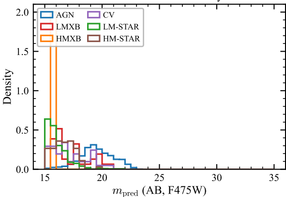
Predicted F475W distribution by class
