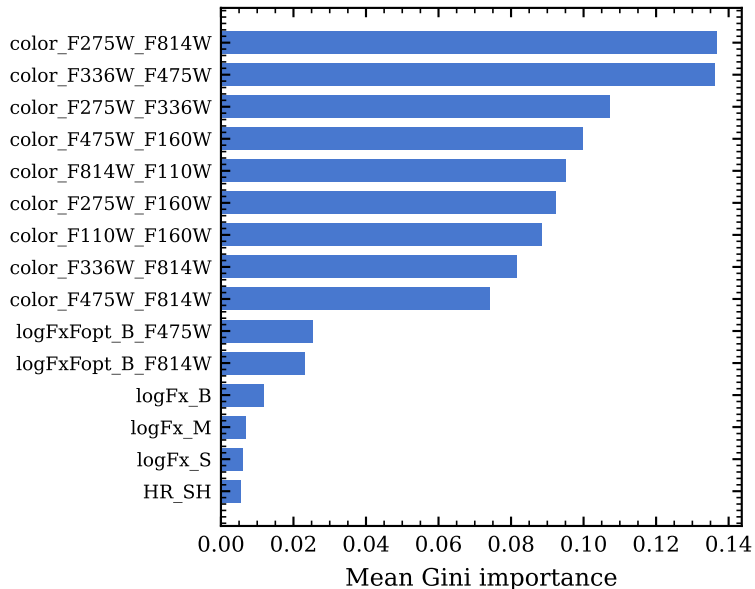
Stage 1 feature importance (top 15)
