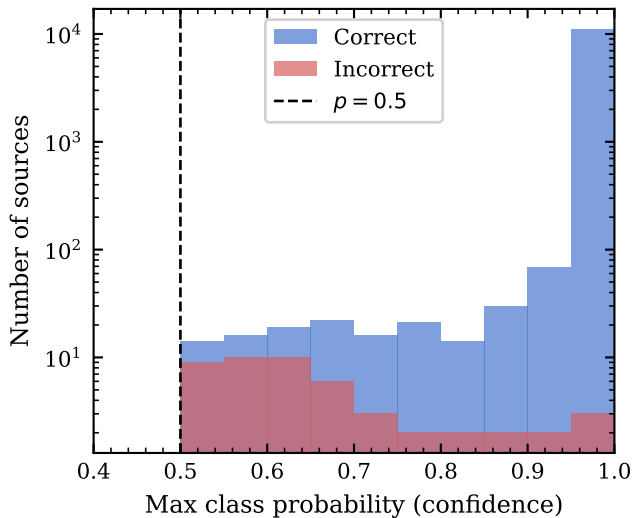
Confidence distribution (full pipeline)
