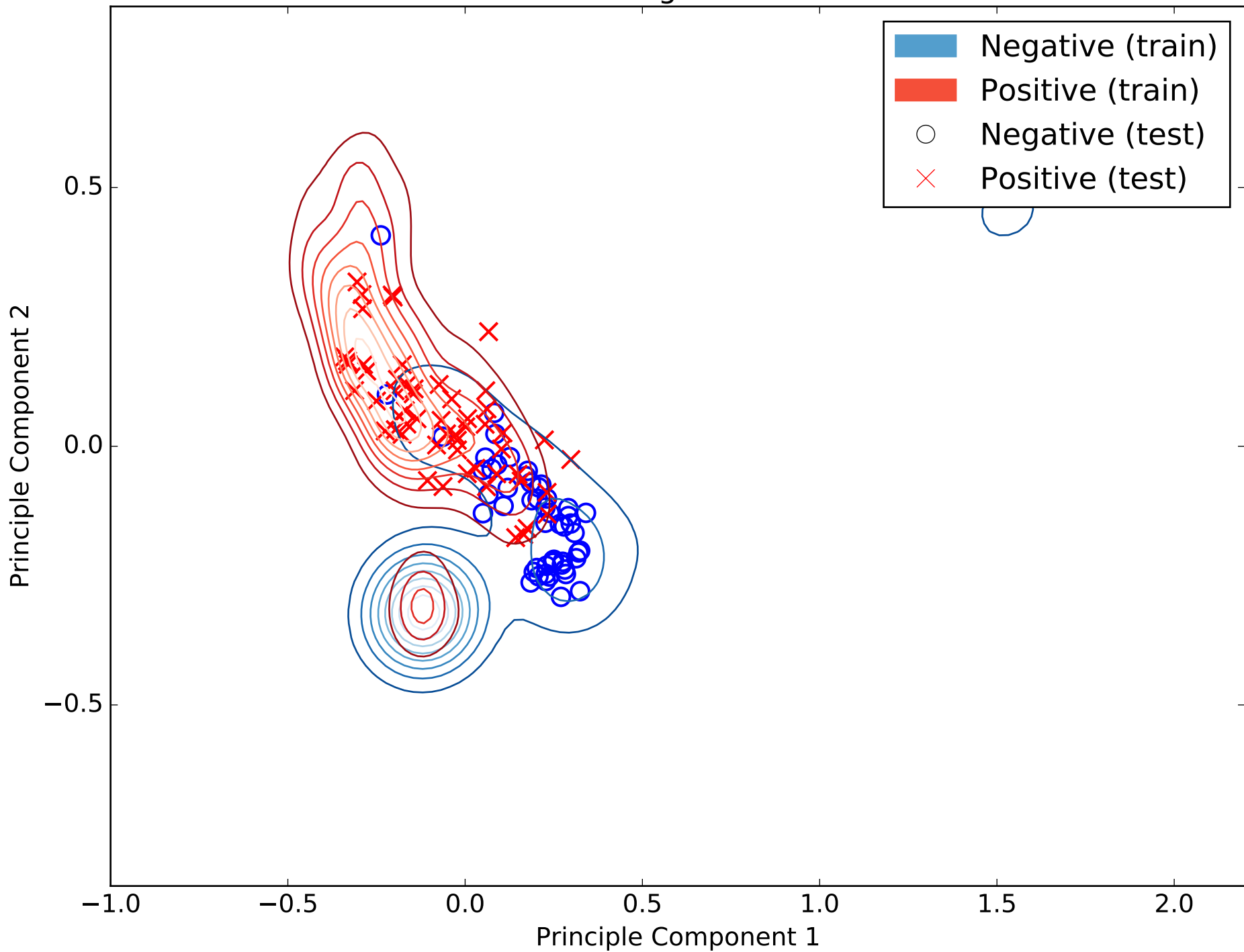
PCA of embeddings for train and test
