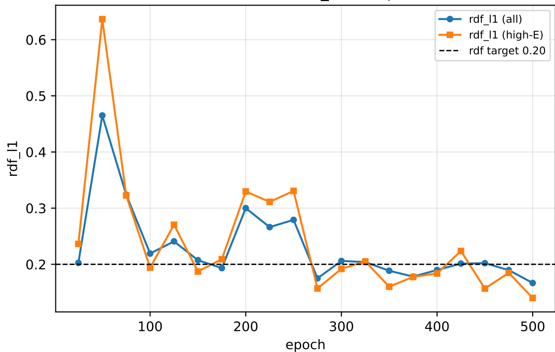
Substructure (rdf_l1) vs epoch
