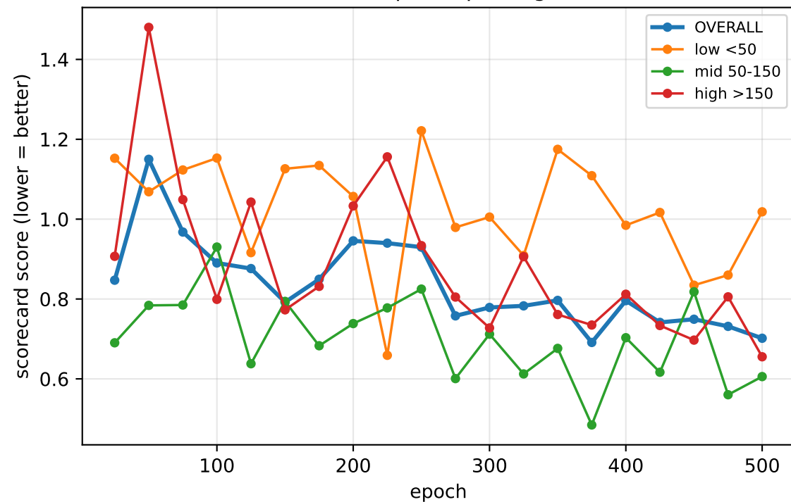
Score vs epoch (per regime)
