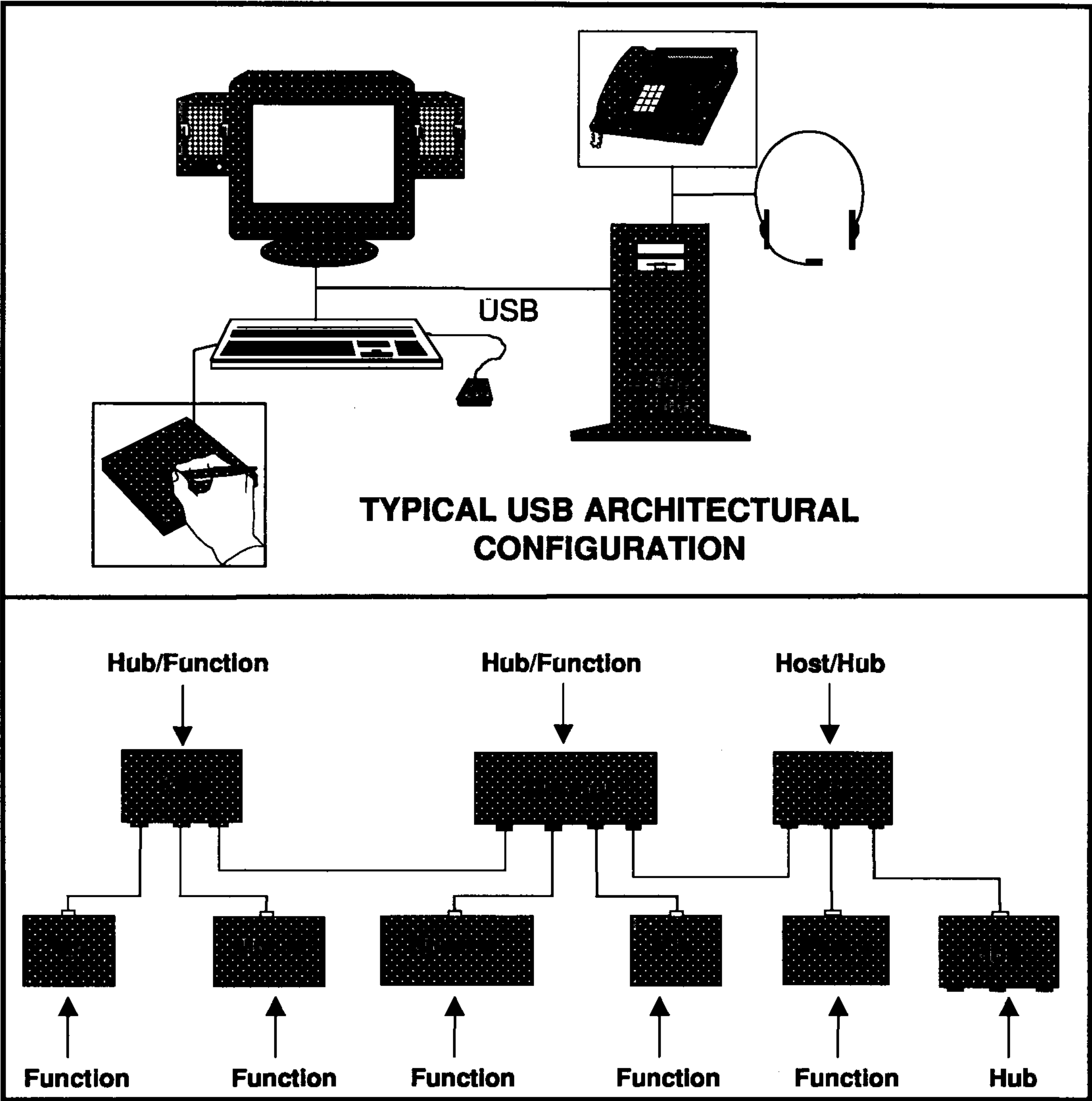
Figure 4-4. Hubs in a Desktop Computer Environment
