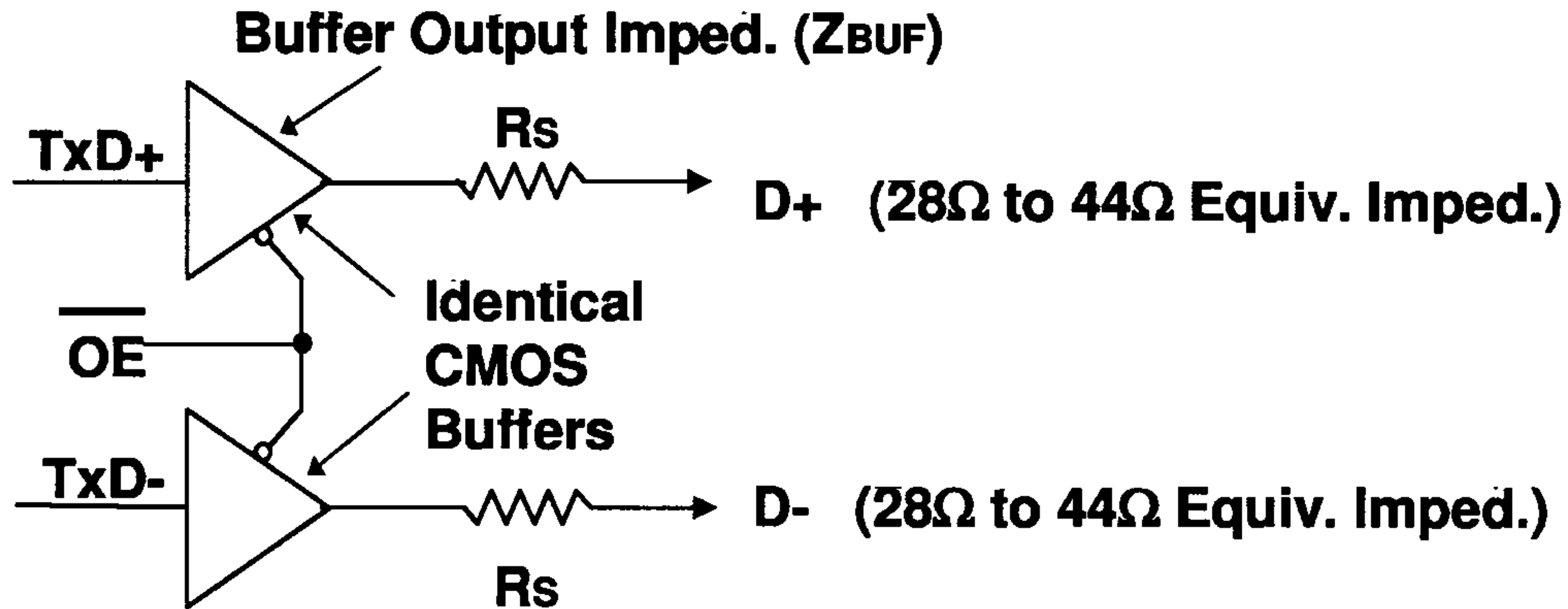
Figure 7-2. Example Full-speed CMOS Driver Circuit
