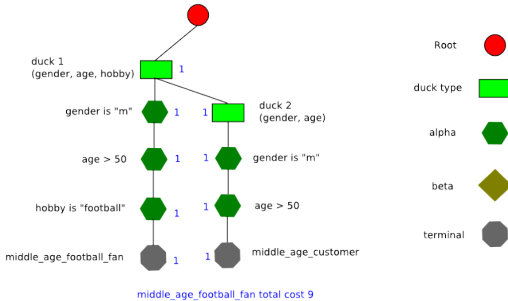
Figure 10.1: Two rules over the duck template compiled without sharing. Each node has cost 1; the join-free rule middle_age_football_fan costs 9 once its share of the type node's successors is counted.
