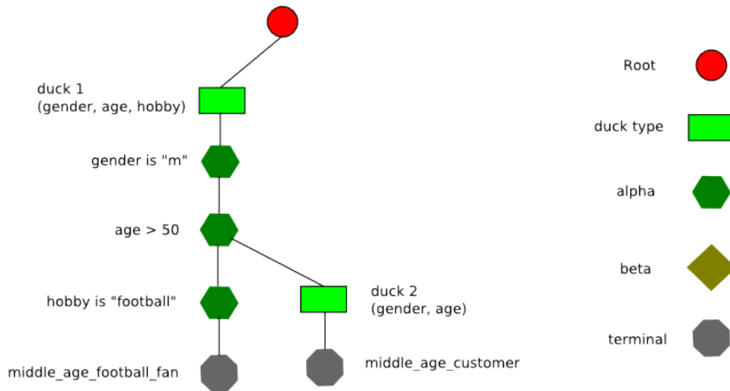
Figure 10.2: The same two rules with alpha-node sharing: gender is "m" and age > 50 are tested once for both.
