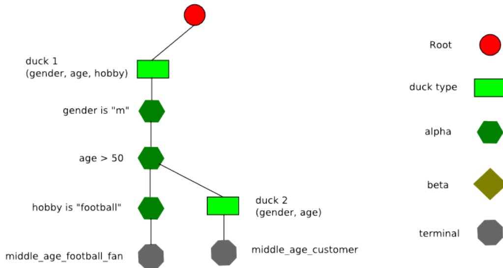
Figure 10.2: The same two rules with alpha-node sharing: gender is "m" and age > 50 are tested once for both.
