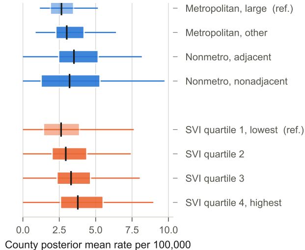
b Absolute scale across counties
