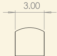
DETAIL C SCALE 5 : 1
