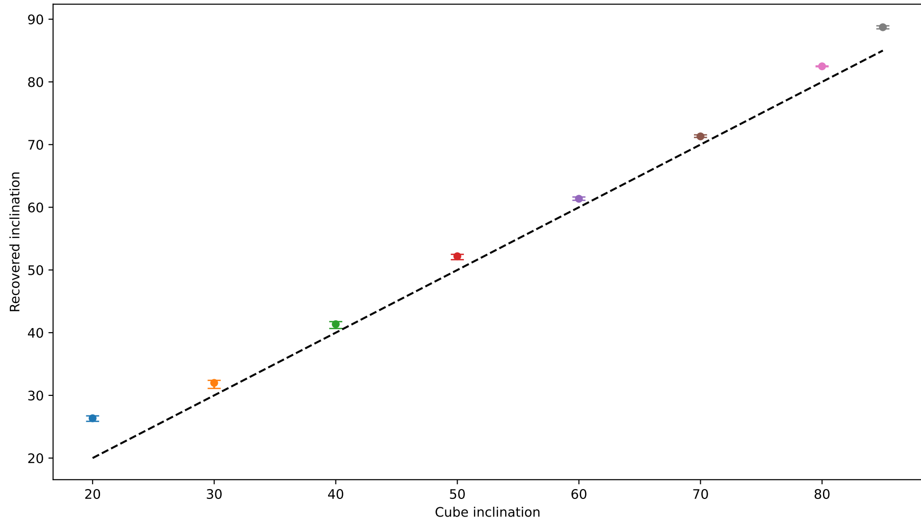
Input vs Recovered Values for Inclinations
