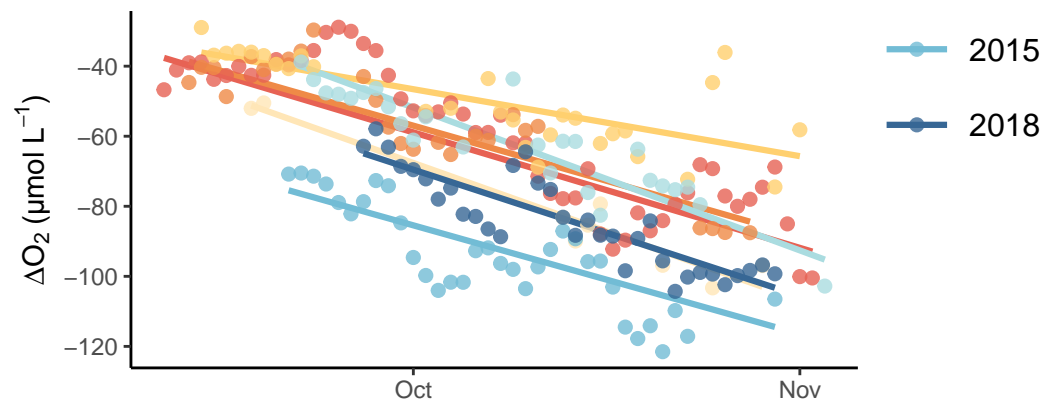
b) \text{O}_2 depletion during leaf loss
