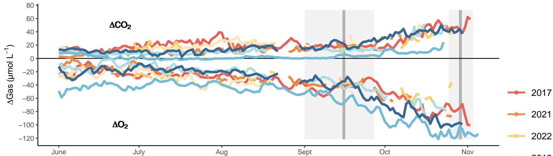
a) Summer and fall gas temporal variation
