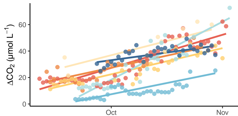
b) \text{CO}_2 accumulation during leaf loss
