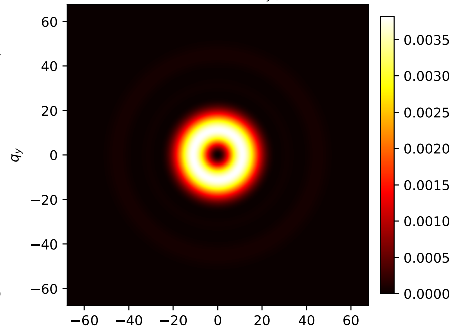
Propagated |E'_x|^2 + |E'_y|^2 + |E'_z|^2
