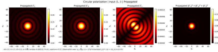
Figure III.4: Base circular, caso (1, i ) (campo propagado).
