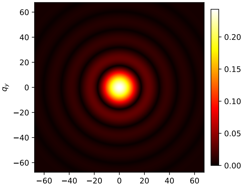
Propagated E'_L
