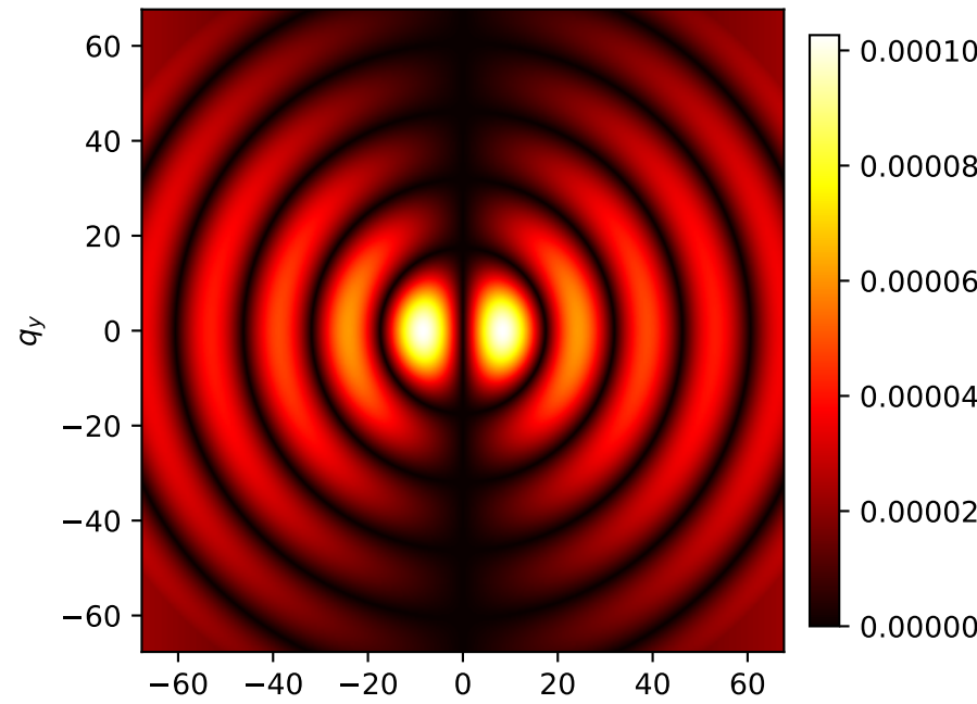
Propagated E'_z
