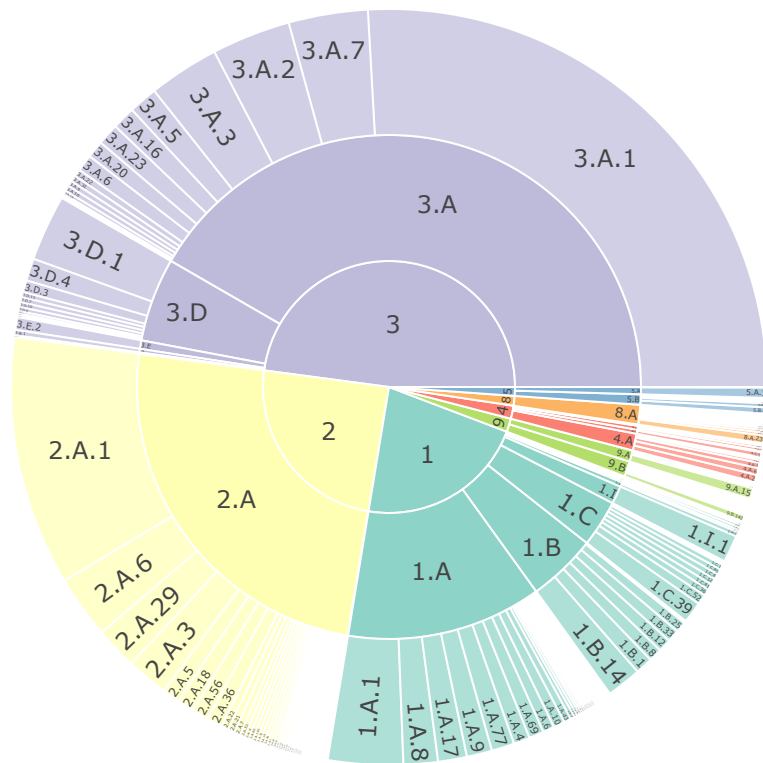
Reactions (9327 transporters)
