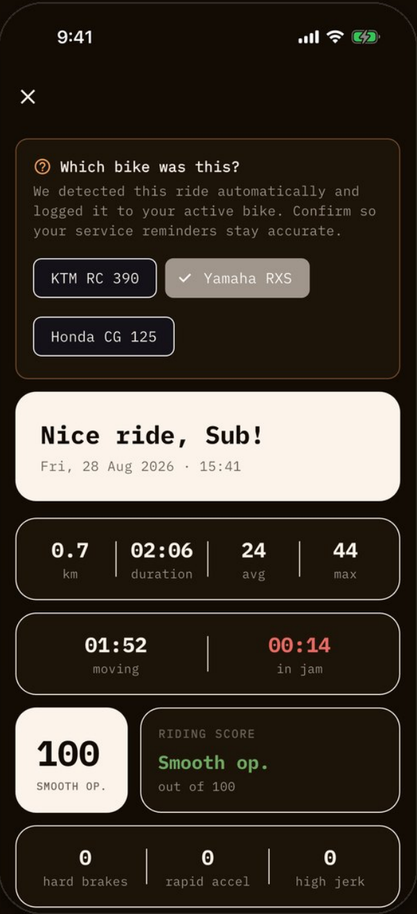
Ride summary
