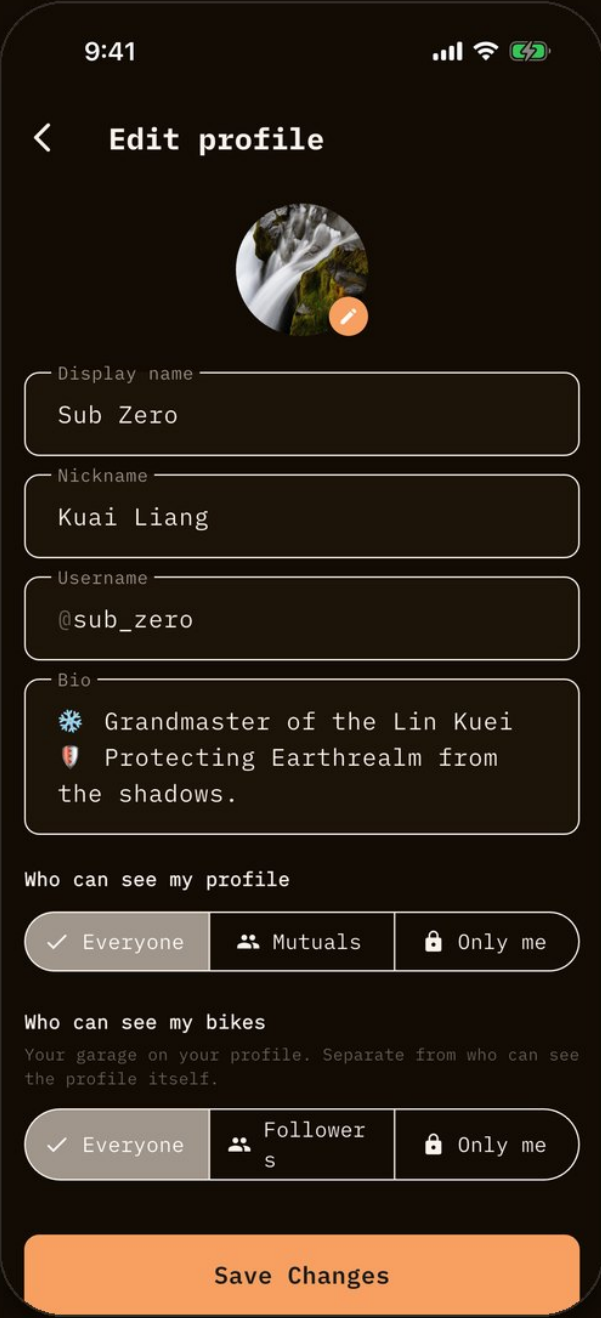
Edit profile
