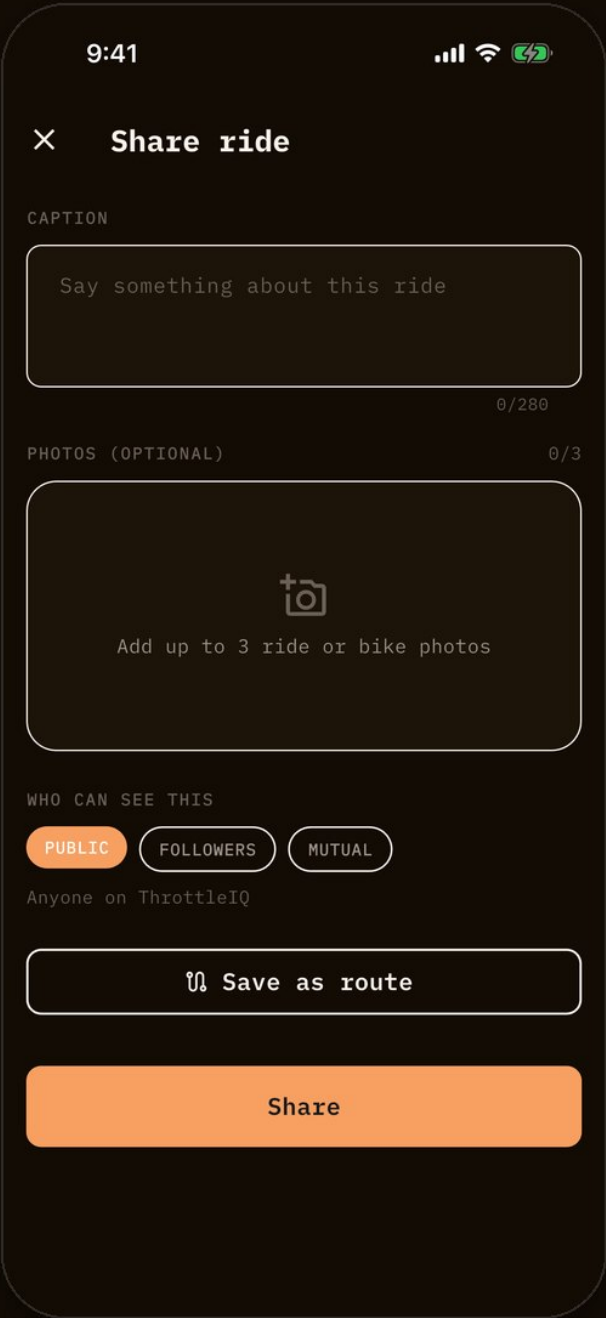
Share ride
