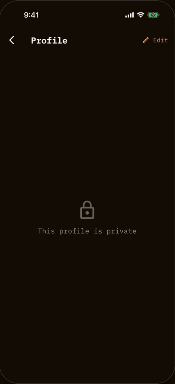
My profile
