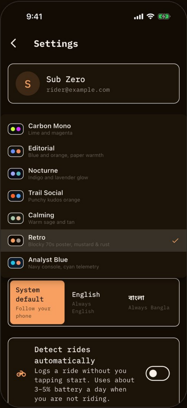
Color picker
