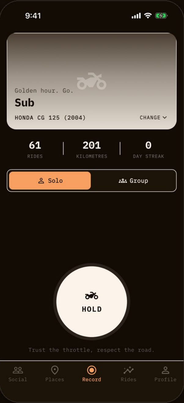
Record dashboard
