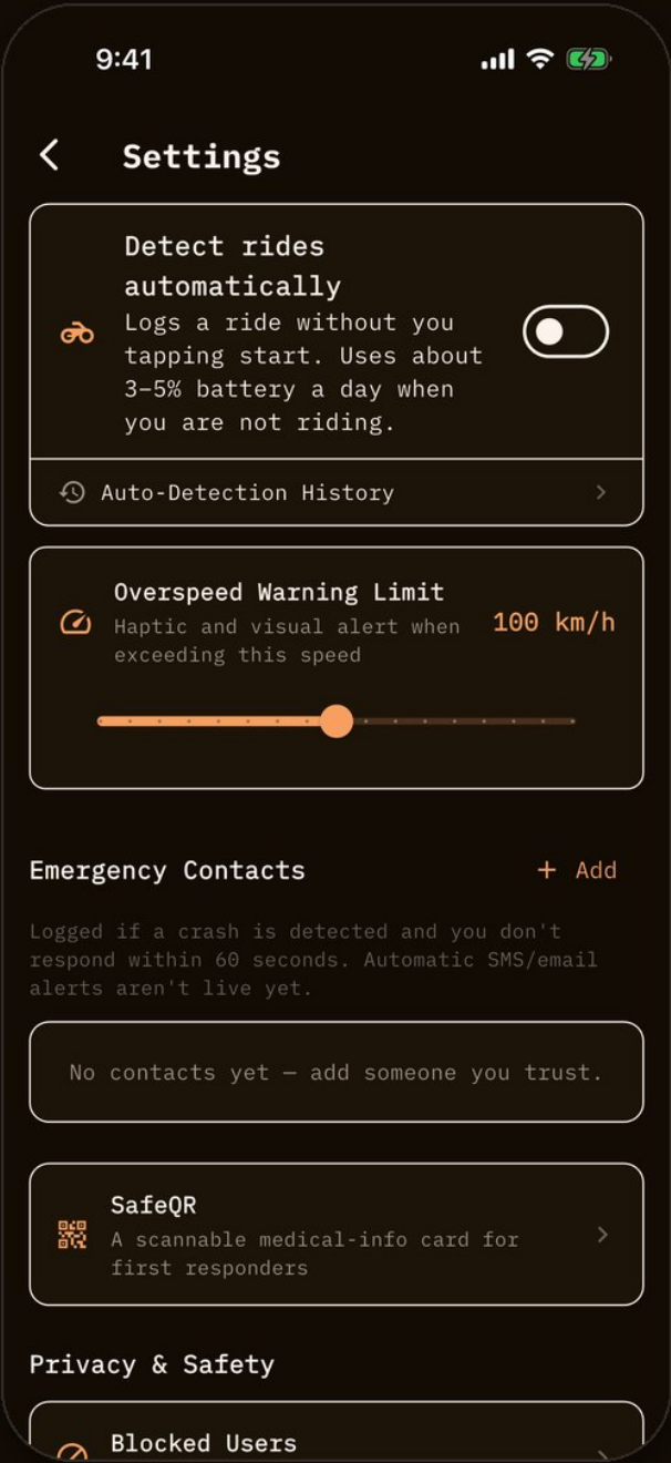
Settings scrolled further (2)
