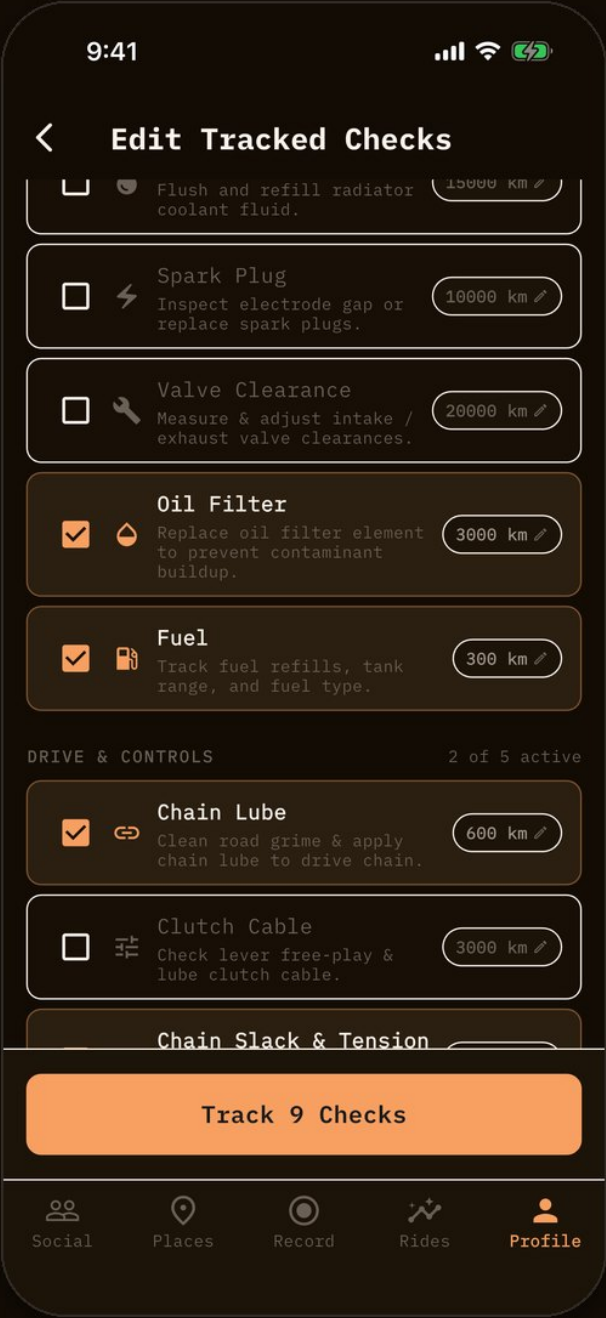
Maintenance schedule scrolled further (2)
