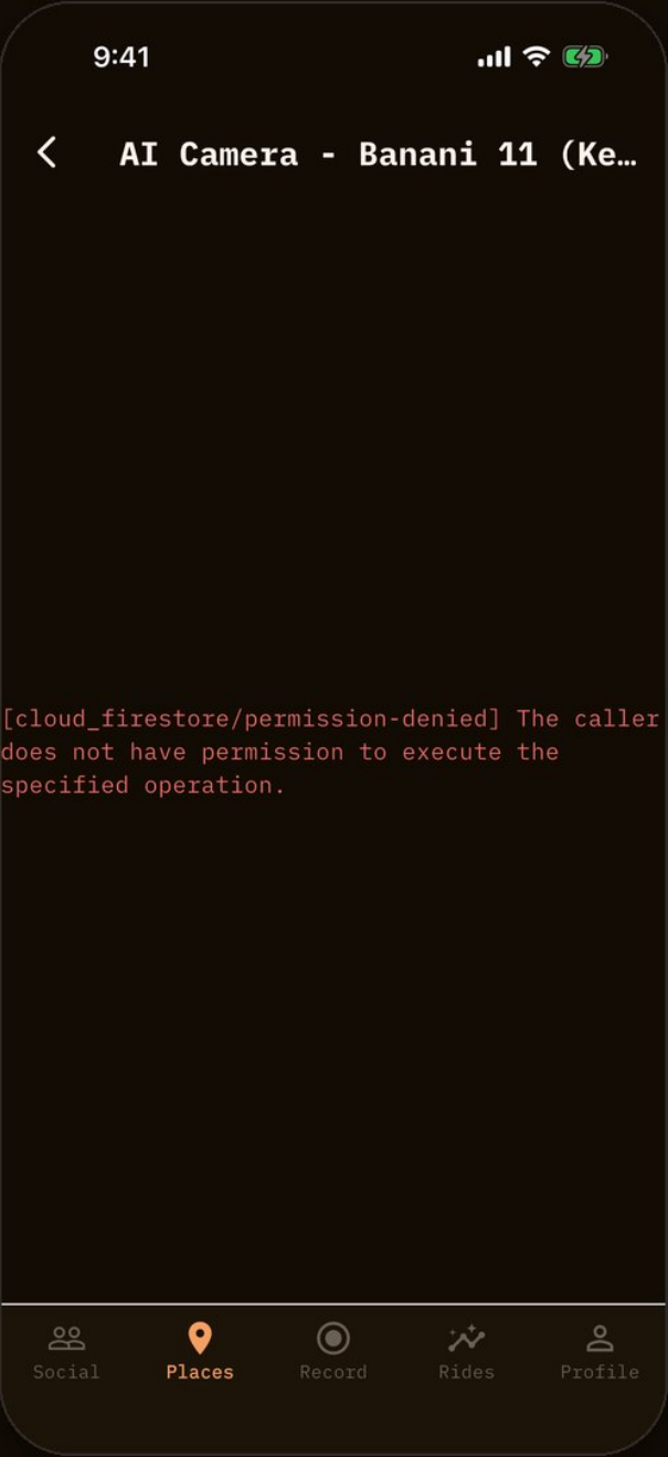
Place detail
