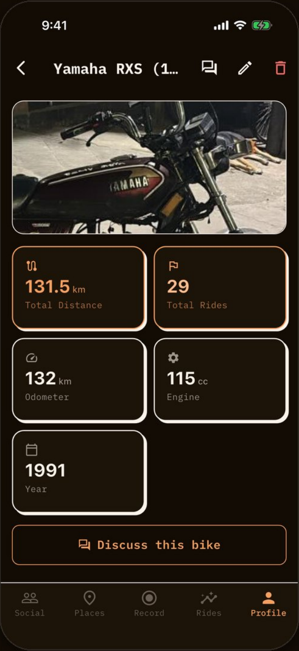
Bike detail
