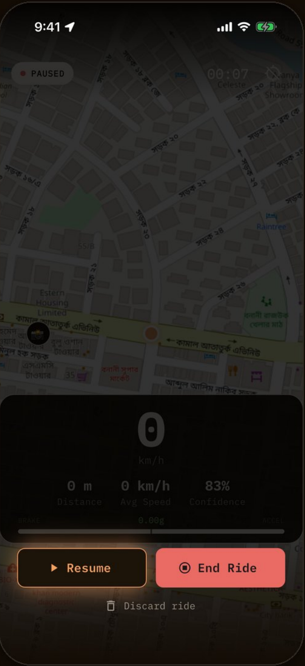
Ride paused
