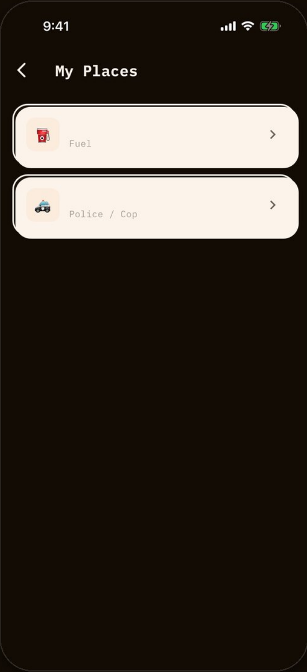
My places
