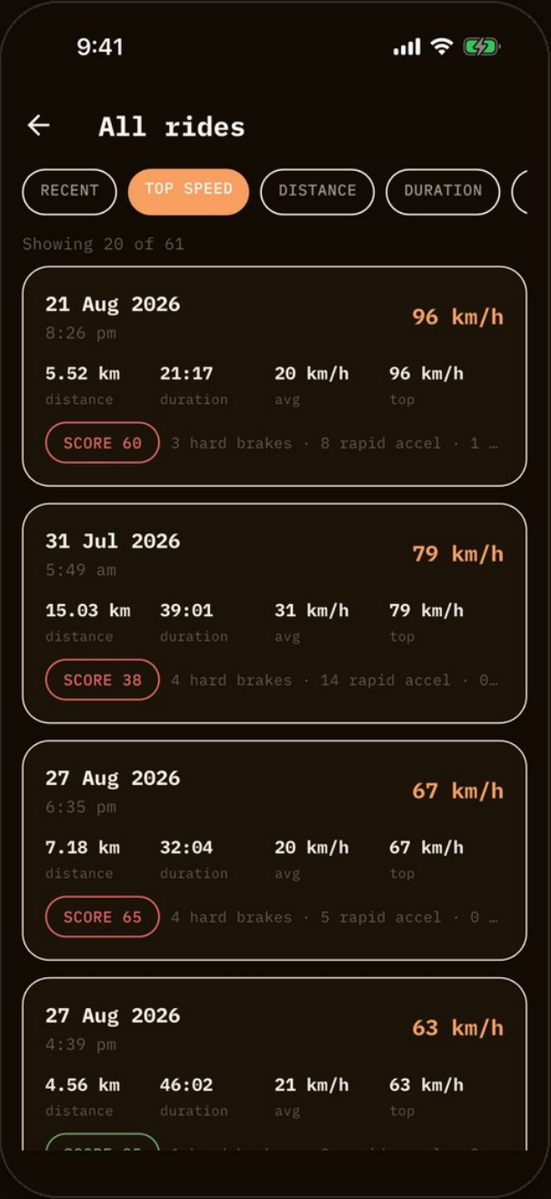
All rides
