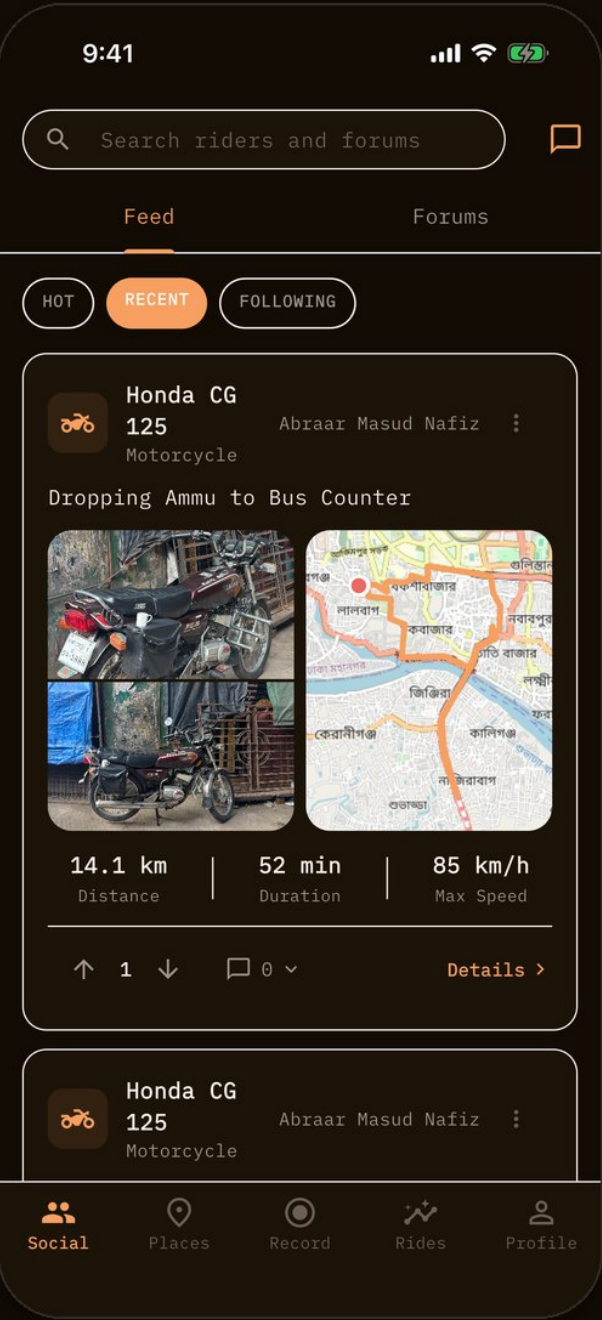
Social feed
