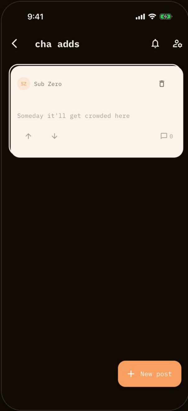
Forum
