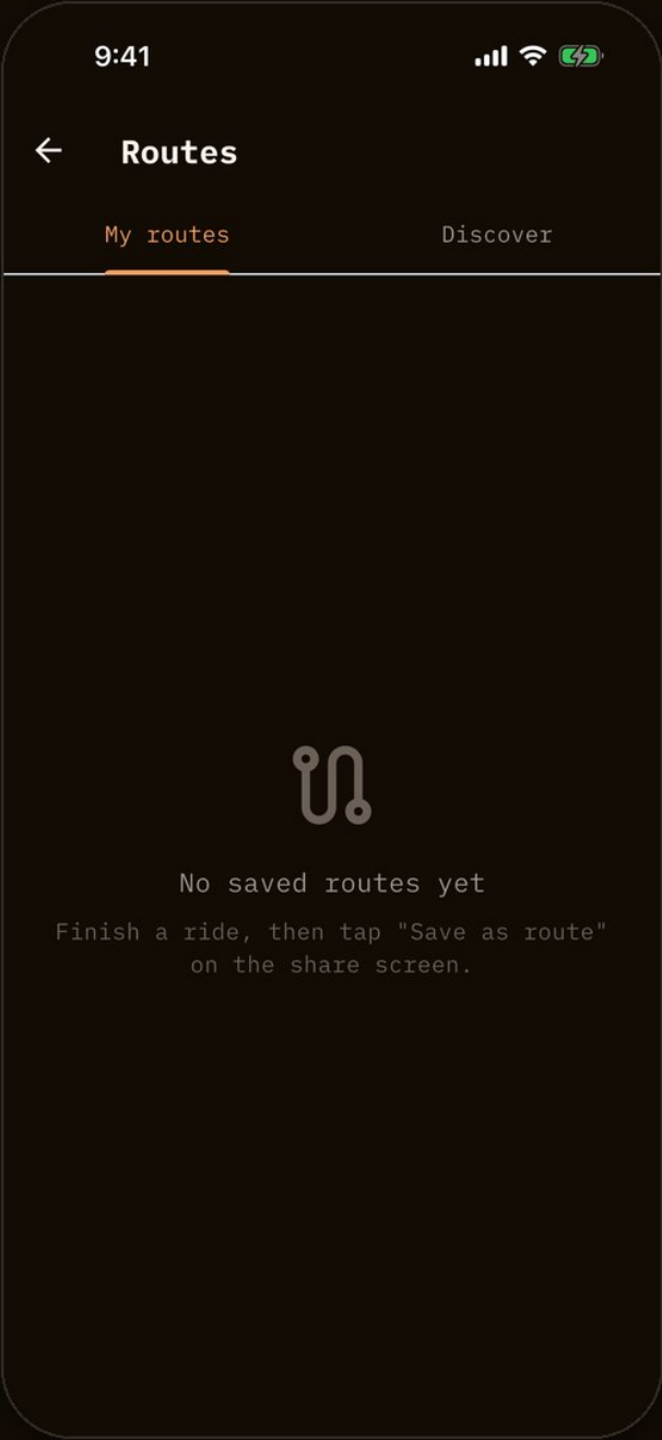
Saved routes
