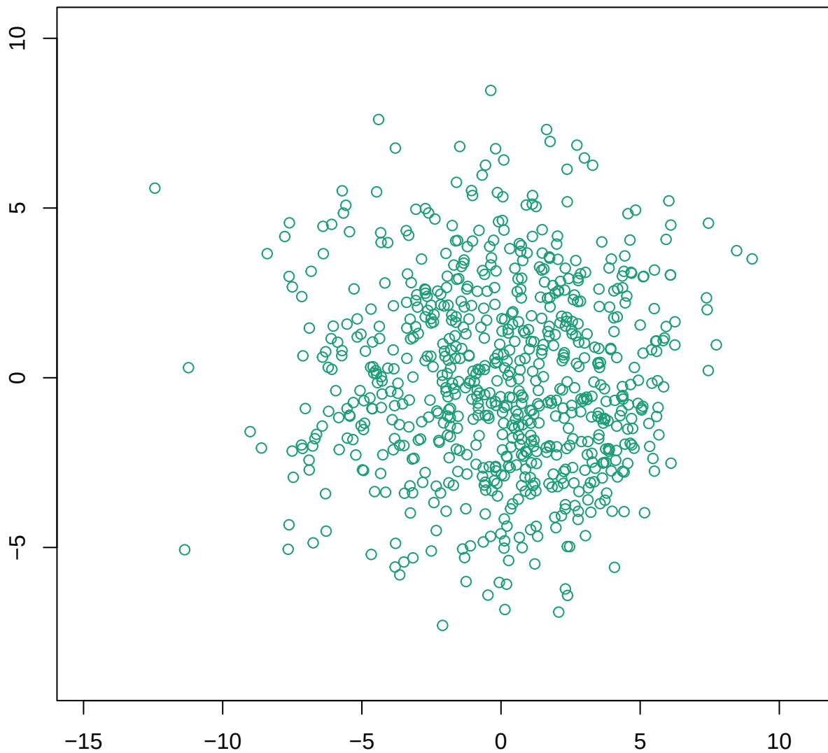
Post-filtering autosomal MDS plot (ungrouped)
