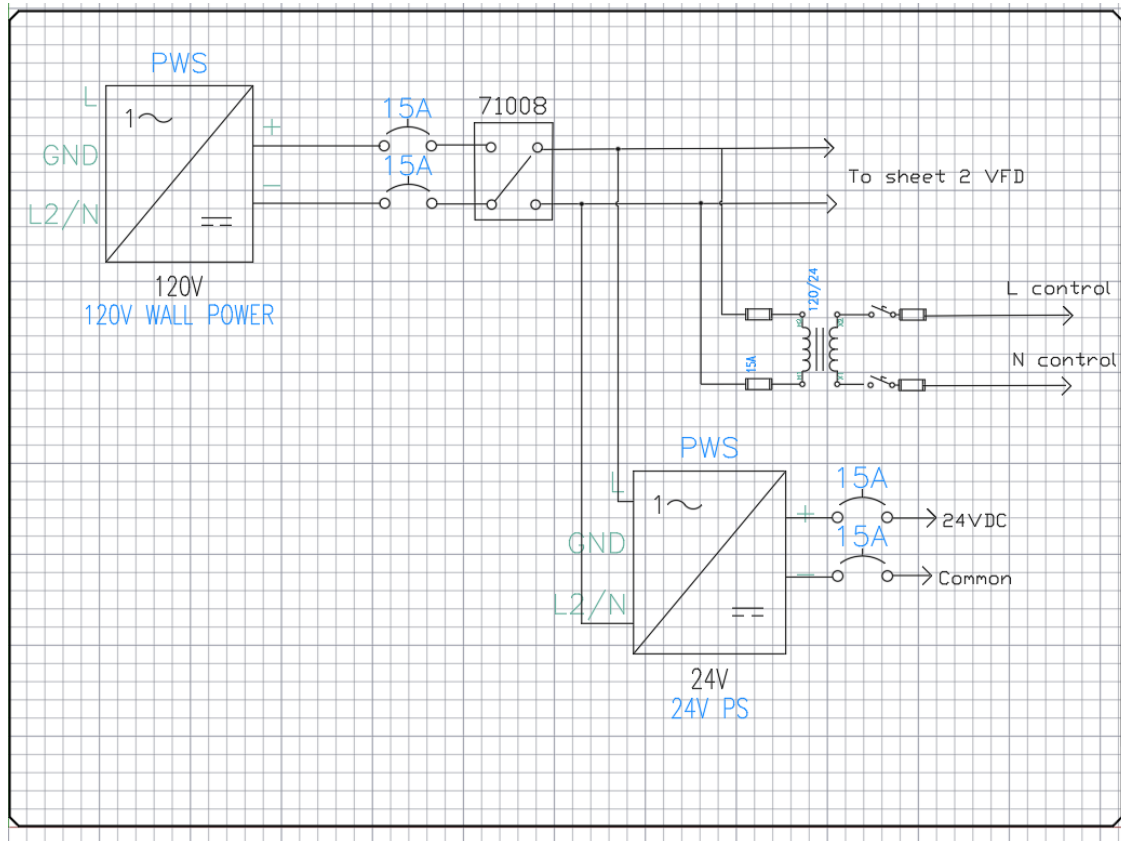
Figure 2: Power distribution circuit: main disconnect, branch breakers, 24 V power supply, and VFD input.
