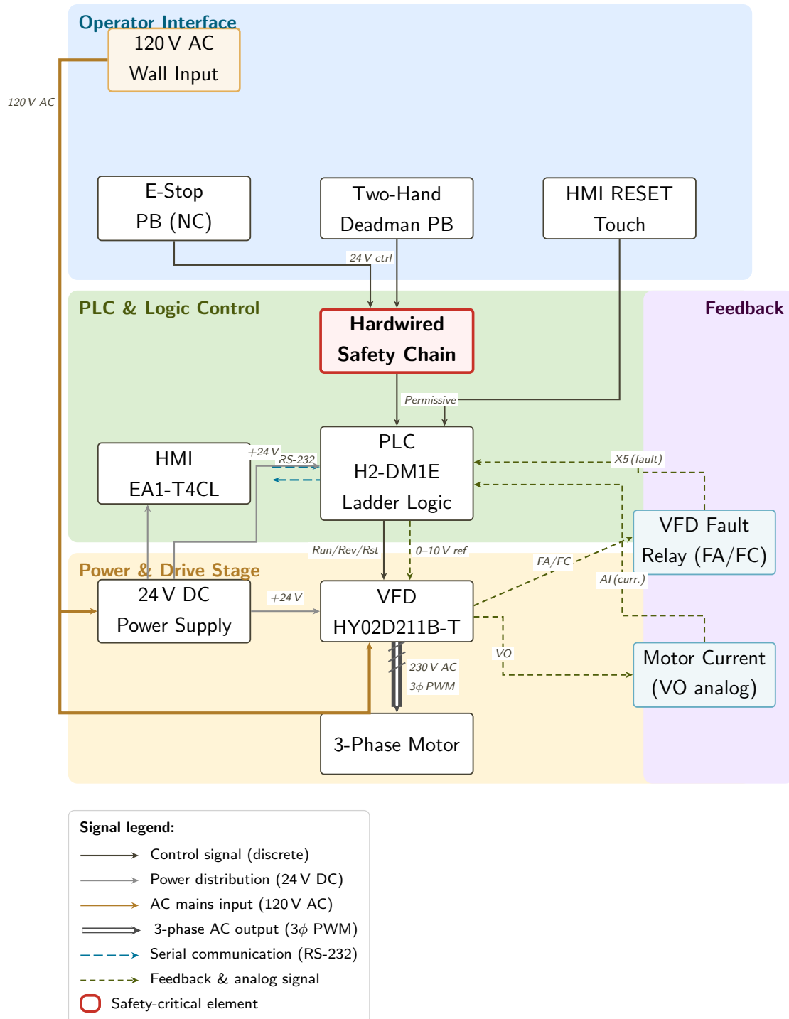
Figure 1: Control system block diagram — signal flow and functional domains.
