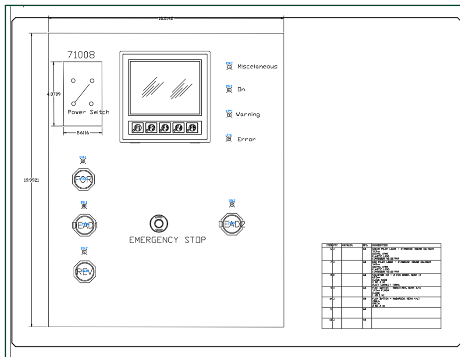
Operator control panel layout
