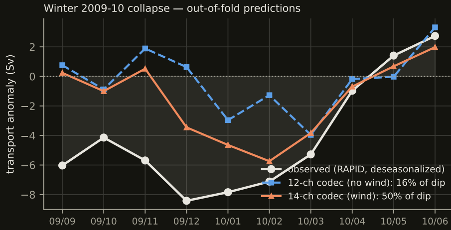
Figure 7: The sharpest event in the RAPID record, predicted out-of-fold. Without wind channels (blue) the model captures 16% of the dip amplitude; with them (orange), 50%. The 25-channel codec reaches 59% (not plotted; see Table 2). The November onset — triggered inside a month — stays invisible to monthly data.
