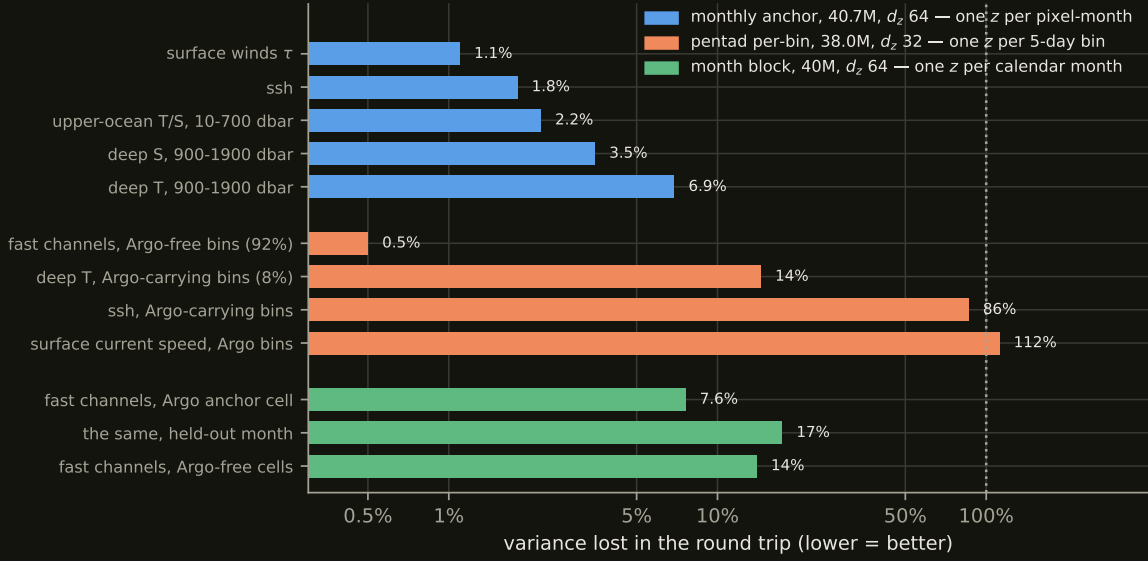
Figure 13: What each codec’s round trip loses , at full visibility — encode and decode with nothing masked and nothing forecast, so this is the representation tax alone. Bars are fraction of channel variance lost ( \text{rmse}^2 in standardized units); the dotted line at 100% is the channel’s own variance, so a bar reaching it carries none of that channel and a constant would have done as well. The monthly anchor is orderly and loses most where the transport integral weights most (deep temperature, 6.9%). The per-bin pentad codec is near-perfect on the 92% of bins that carry no Argo and collapses on the 8% that do — 40 channels competing for 32 latent dimensions. The month-block codec cures that collapse at the anchor and pays a flat structural price everywhere else: one embedding per month is a genuine \approx 4:1 squeeze in time.
