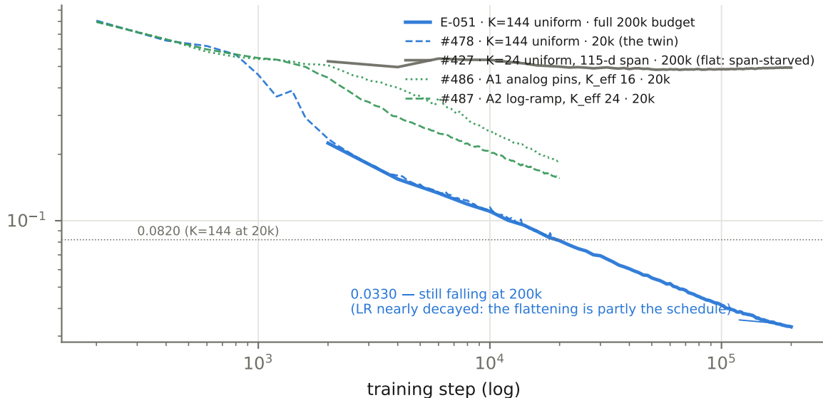
Pentad one-step vs training budget: the full-budget K=144 curve is NOT saturated; K=24 is span-starved flat
