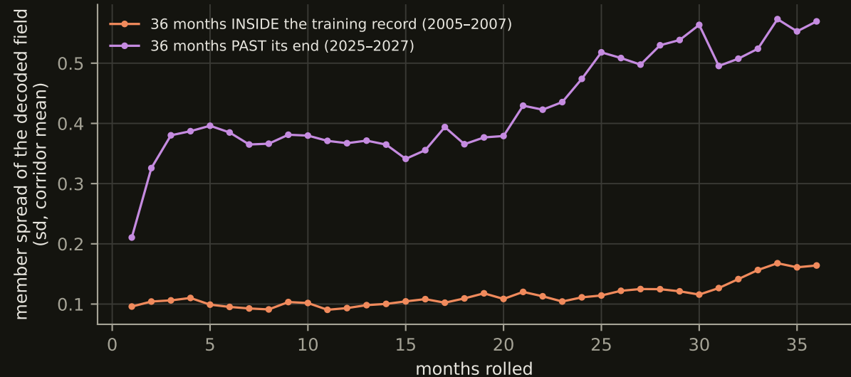
8-member ensemble, contaminated head (run #513): confident where it memorised
