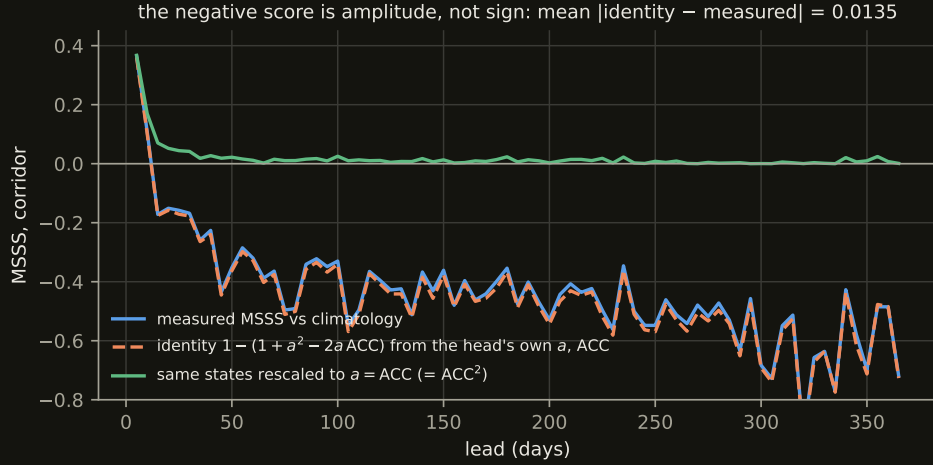
Figure 5: Measured corridor \text{MSSS}_{\text{clim}} per lead for the clean head, the value the identity predicts from the head’s own ACC and amplitude ratio, and the value the same states would score rescaled to a = \text{ACC} .
