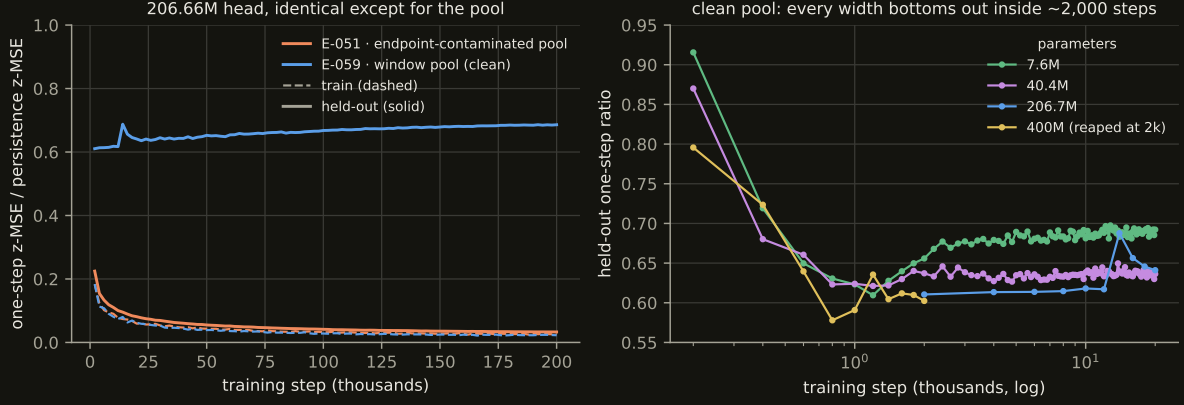
Figure 2: Left: one-step z -space MSE relative to persistence, training (dashed) and held-out (solid), for the 206.66M head under the contaminated pool (E-051) and the corrected pool (E-059) — same architecture, seed, codec, embedding, validation windows and hardware. Right: the held-out ratio over the first 20,000 steps for four widths under the corrected pool.
