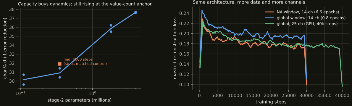
Figure 13: Left: the original stage-2 capacity sweep (0.11–4M parameters, 12-channel coarse tensor, no stencil) — the first sign, in retrospect, that stage-2 capacity was the binding axis; it was still rising at its top end. Right: codec training curves across generations.
