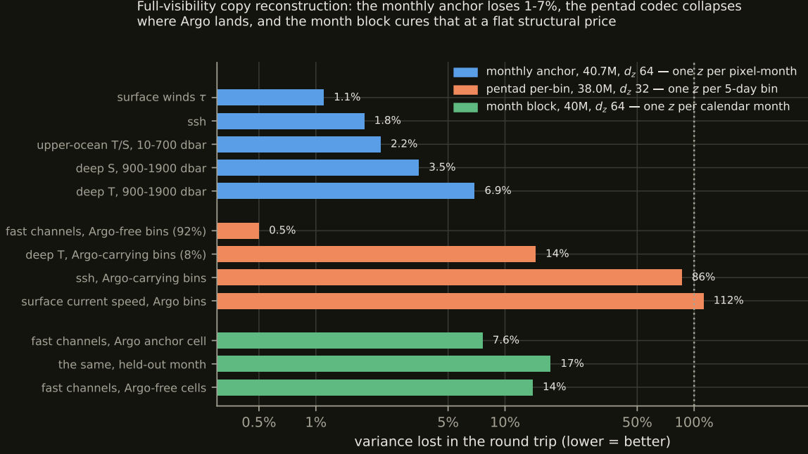
Figure 12: What each codec’s round trip loses , at full visibility — encode and decode with nothing masked and nothing forecast, so this is the representation tax alone. Bars are fraction of channel variance lost ( \text{rmse}^2 in standardized units); the dotted line at 100% is the channel’s own variance, so a bar reaching it carries none of that channel and a constant would have done as well. The monthly anchor is orderly and loses most where the transport integral weights most (deep temperature, 6.9%). The per-bin pentad codec is near-perfect on the 92% of bins that carry no Argo and collapses on the 8% that do — 40 channels competing for 32 latent dimensions. The month-block codec cures that collapse at the anchor and pays a flat structural price everywhere else: one embedding per month is a genuine \approx 4:1 squeeze in time.
