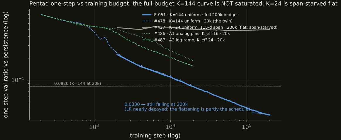
Figure 13: Pentad one-step against training budget , every curve the in-training validation ratio against the shared persistence baseline (21.44621). The full-budget K=144 head (E-051) is a clean power law to 200k with no saturation — and its terminal flattening is partly the LR schedule (half-life 40k, so the rate is 1/32 of peak by 200k), not the model. The same budget bought K=24 nothing ( 0.506 \rightarrow 0.494 over 10\times the steps: span-starved), which is the budget \times span interaction in one picture. The sparse-time arms (A1, A2) track between. This figure is why the continuation and capacity arms (§10.3) are worth their price.
