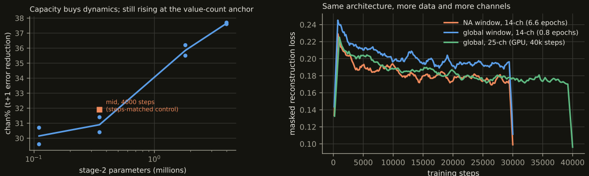
Figure 20: Left: the original stage-2 capacity sweep (0.11–4M parameters, 12-channel coarse tensor, no stencil) — the first sign, in retrospect, that stage-2 capacity was the binding axis; it was still rising at its top end. Right: codec training curves across generations.
