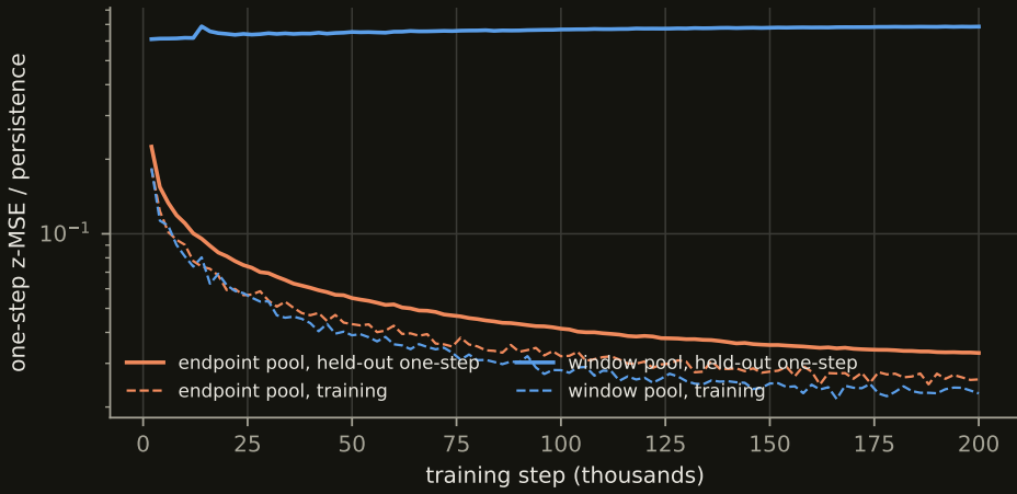
Figure 19: Training and held-out one-step loss of the 206.7M pentad head under the two pools, as a fraction of the persistence error.
