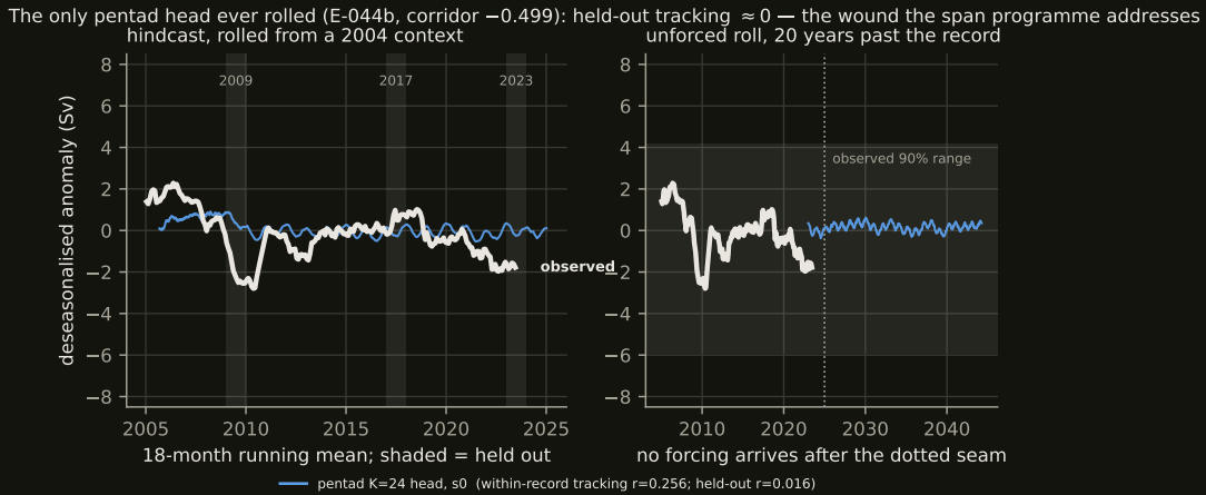
Figure 14: The transport read-out of the only pentad head ever rolled — E-044b's K=24 , 115-day-span head, whose day-matched corridor AUC is -0.499 , below climatology. Its within-record tracking is 0.256 and its held-out-year tracking 0.016 — effectively decoupled from the observed series, the transport view of the pentad wound. The model curve is smoothed over the concatenated record+future series, so the prediction continues seamlessly across the end of the measurements. No frontier pentad head has a roll yet: E-051's (0.0330 one-step) is the registered decisive reading and the E-053 offset heads are refused by the evaluator until the replay battery and offset-aware assembly exist.
