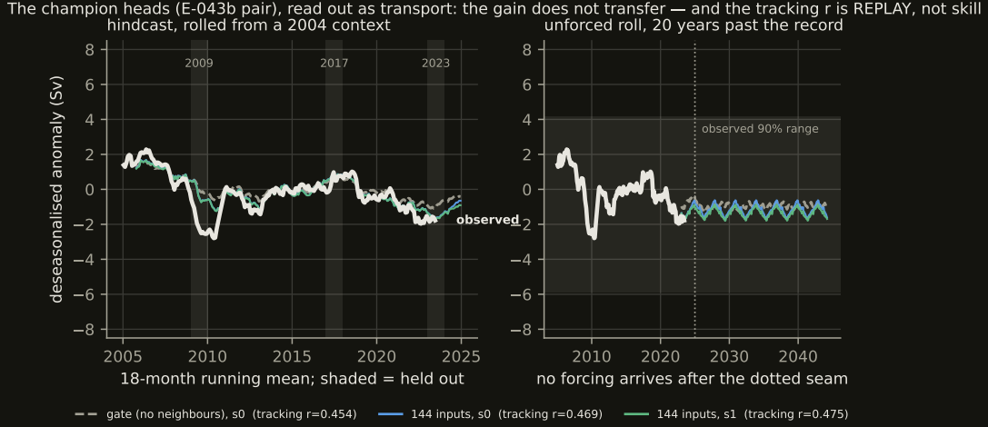
Figure 10: The AMOC read-out of the champion heads — the E-043b no-longitude-holdout pair, the best rolled configuration on record (corridor AUC 0.93733/0.93758, both seeds shown) — against the frozen no-neighbour gate. (The frontier pentad head of §10.3, one-step 0.0330, has no roll yet; this figure shows the best heads that have been rolled.) Left: hindcast from a 2004 context, with the three never-trained years shaded. Those columns are not a test, and the legend’s r is not a skill number: §9.2 rolls this configuration from six context ends spanning a decade and finds the tracking correlation flat in lead time and the post-record peaks pinned to fixed calendar months whatever the starting state. The whole left panel — shaded columns included — is trajectory replay, and its r is relabelled here as replay tracking: it measures how completely the head has memorized the record, not how well it forecasts. Right: twenty years of unforced roll past the end of the record. The flatness on the right is the finding, not a forecast: with no wind or heat-flux forcing after the seam, the learned dynamics relaxes toward climatology and stops moving, which is a damped attractor rather than a quiet ocean — and §9.2 adds that what residual motion there is repeats on an integer number of years. Interactive version, with the per-arm table, at blauewelt.github.io/earth/ml/paper/figs/amoc.roll.html .
