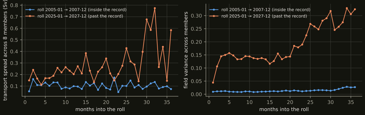
Figure 18: Ensemble dispersion of the 8-member stencil head over a 36-month roll inside and past the training record.
