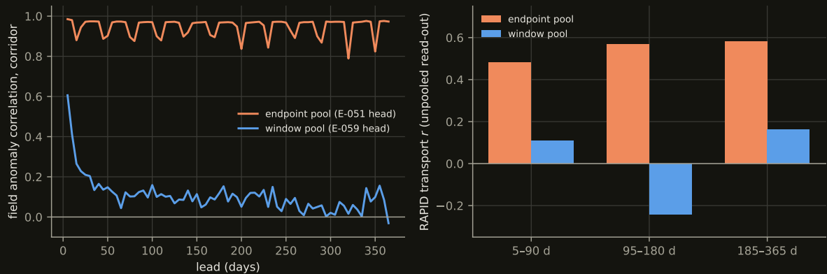
Figure 16: The same rolled battery under the two pools. Left: corridor field anomaly correlation against lead. Right: unpooled RAPID transport correlation by lead band.
