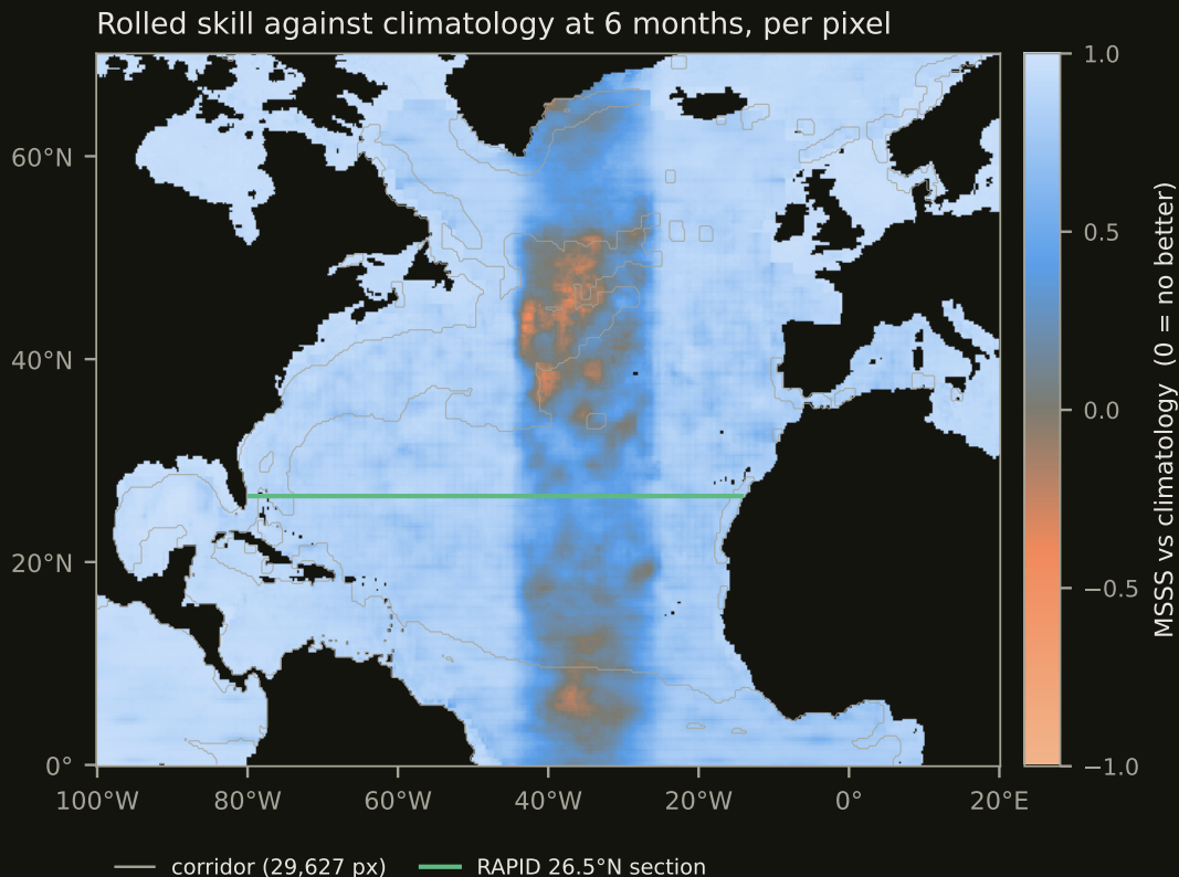
Figure 7: Where the rolled skill sits. Per-pixel MSSS against climatology at a six-month horizon — pooled over all 39 channels and every evaluation start-month — for all 84,405 window pixels. Positive means beating the train-month climatology, zero means matching it, and the colour scale is symmetric about zero, so the midpoint is the climatological line itself. Land and out-of-window cells are blank: an unmodelled cell and a zero-skill cell are not the same thing. Grey: the 29,627-pixel corridor, whose outline follows the coast almost everywhere because the fastest quarter of the window largely is coastal. Green: the 265-pixel RAPID 26.5°N section (80°W–13°W), where the transport read-out is taken. The head is e032x1_u1_s0.pt — sunflower-144 at 1024 \times 16 , seed 0 — from run #356, staged in the repository as m1/paper/roll.356.json ; the pixels carry no coordinates in that file, and their geography is recovered from data/amoc_eval_mask.json , which the evaluator writes from the same ys/xs arrays it scores. This is one seed , and the figure is here to show where the skill sits rather than to quote a level; the seed-averaged corridor AUC of Table 5 remains the number.
